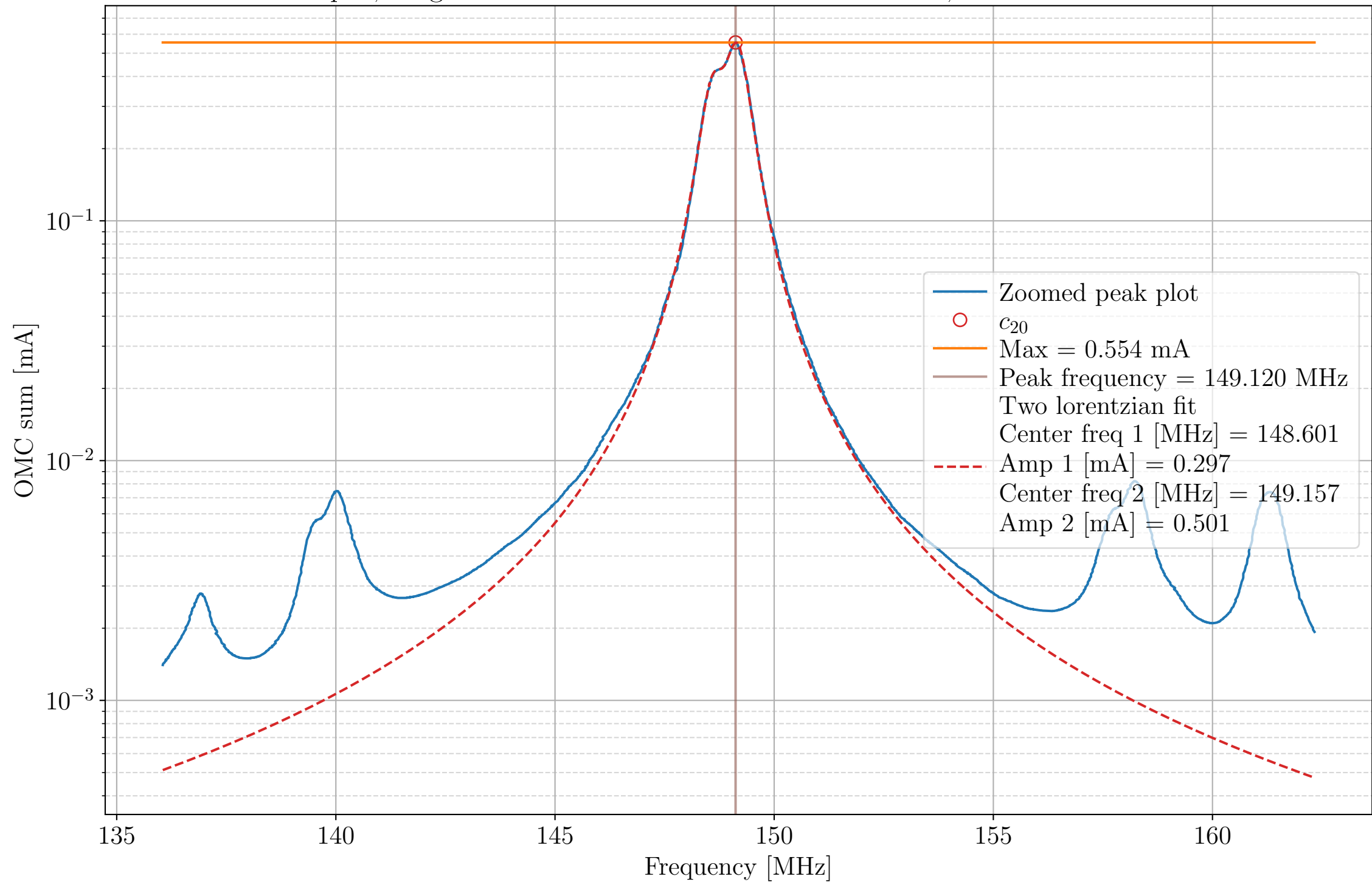
10W input, Single bounce ITMX zoomed at carrier + 20, HWHM = 0.335 MHz
