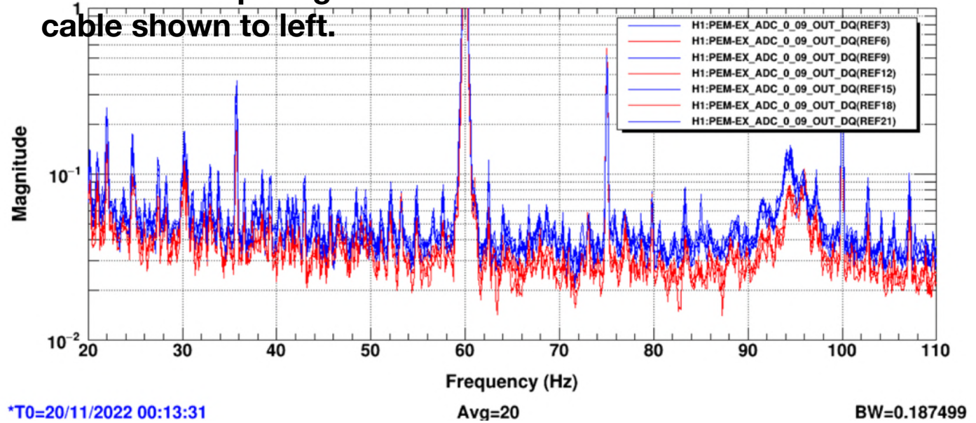
Ground cable connected to racks, and chassis (including ESD) cable tray, beam tube
