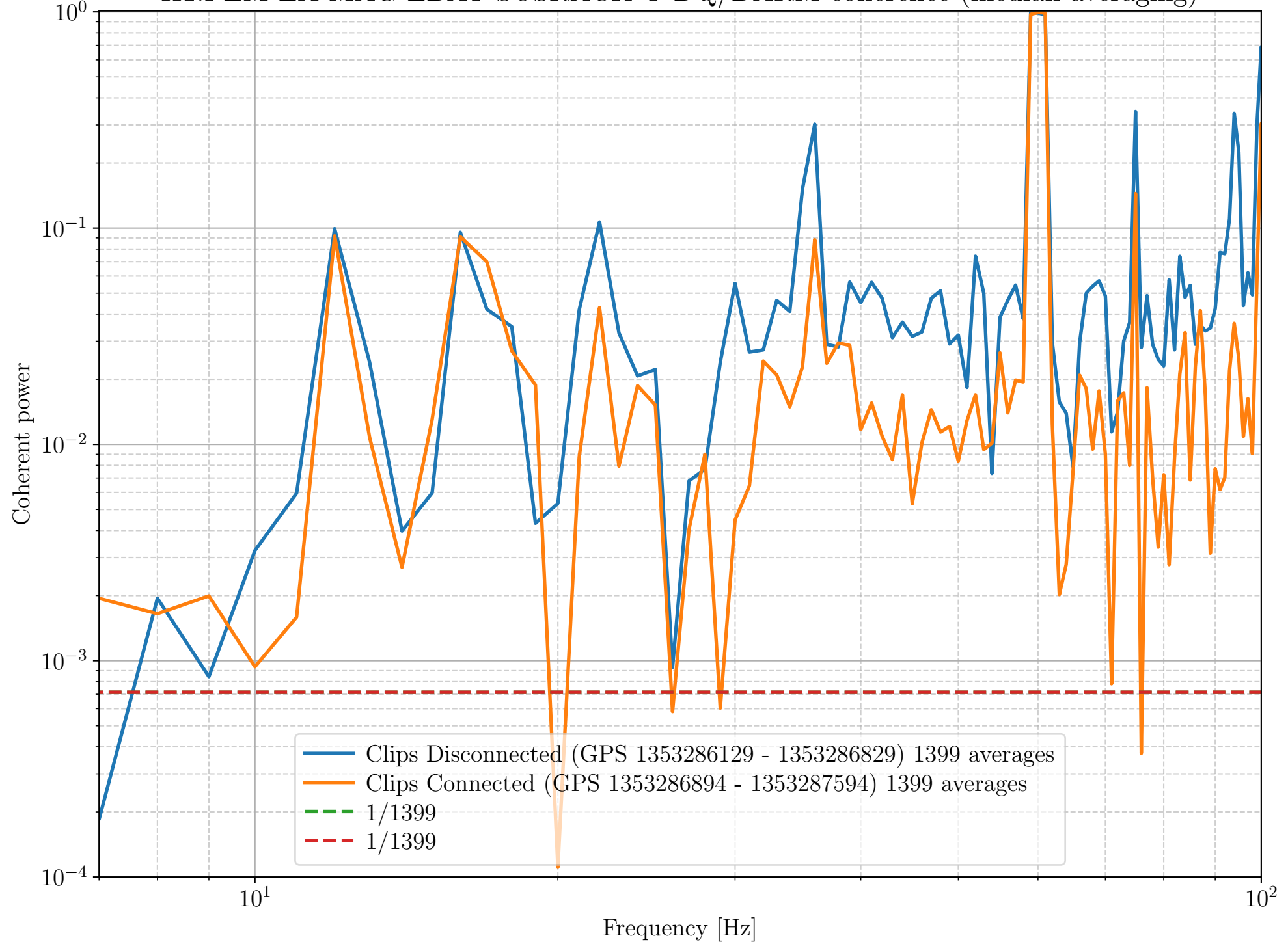
H1:PEM-EX MAG EBAY SUSRACK Y DQ/DARM coherence (median averaging)
