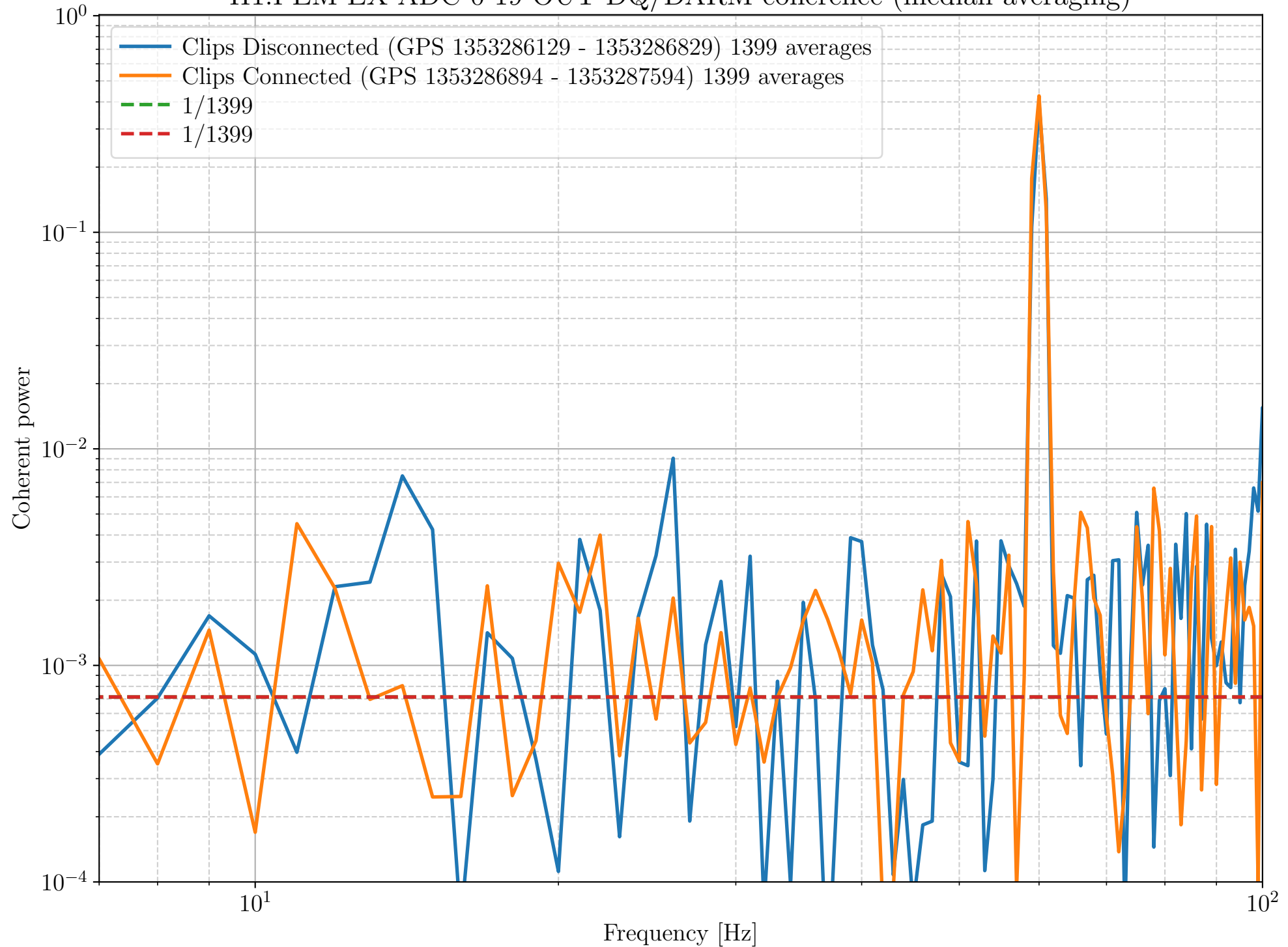
H1:PEM-EX ADC 0 19 OUT DQ/DARM coherence (median averaging)
