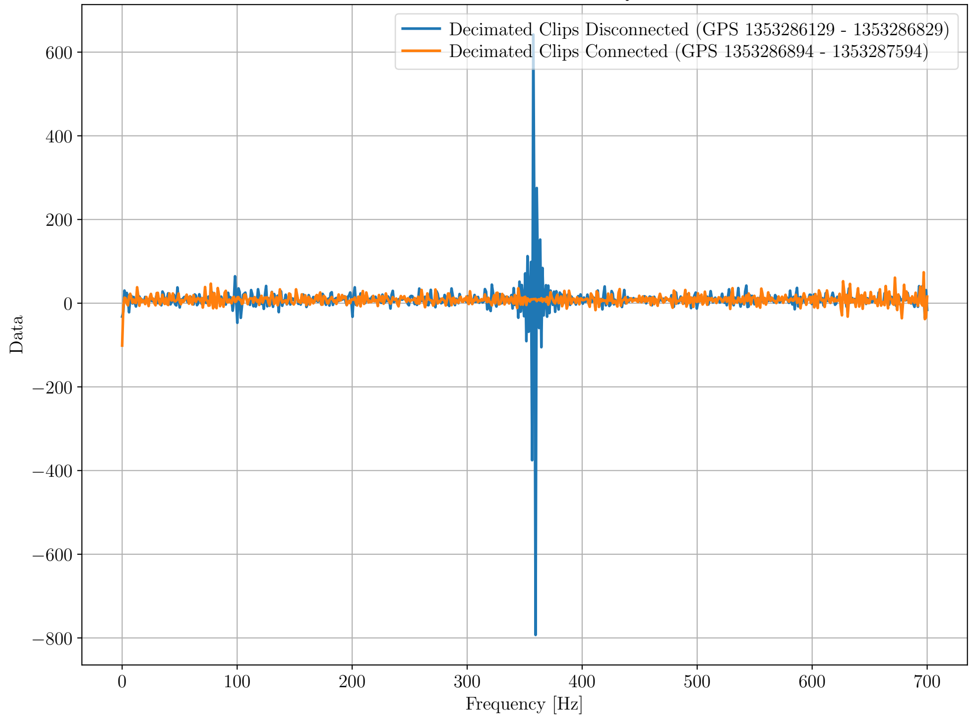
H1:PEM-EX MAG EBAY SUSRACK Y DQ decimated time series
