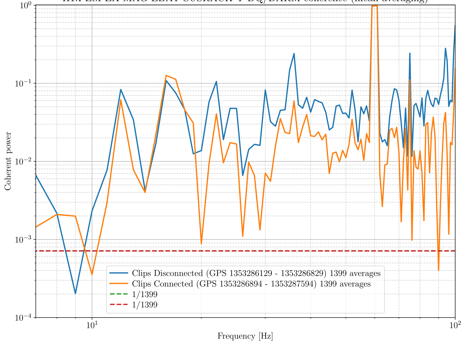
H1:PEM-EX MAG EBAY SUSRACK Y DQ/DARM coherence (mean averaging)
