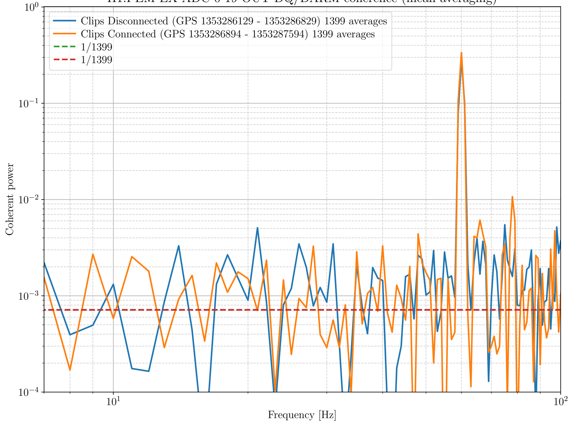
H1:PEM-EX ADC 0 19 OUT DQ/DARM coherence (mean averaging)
