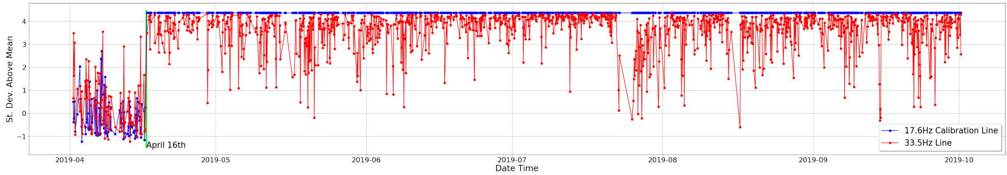
Figure 4: O3 A Calibration Line to 33.5Hz line Comparison
