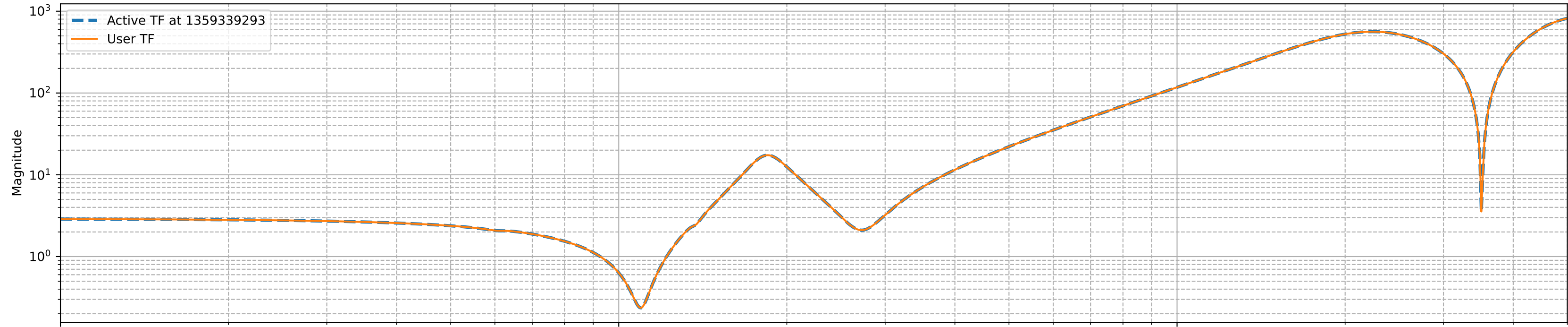
H1:ASC-RPC CHARD Y Active TF at gpstime = 1359339293 FMs engaged: 1 3 4 5 6 7, gain = 3.50, input = 1 output = 1
