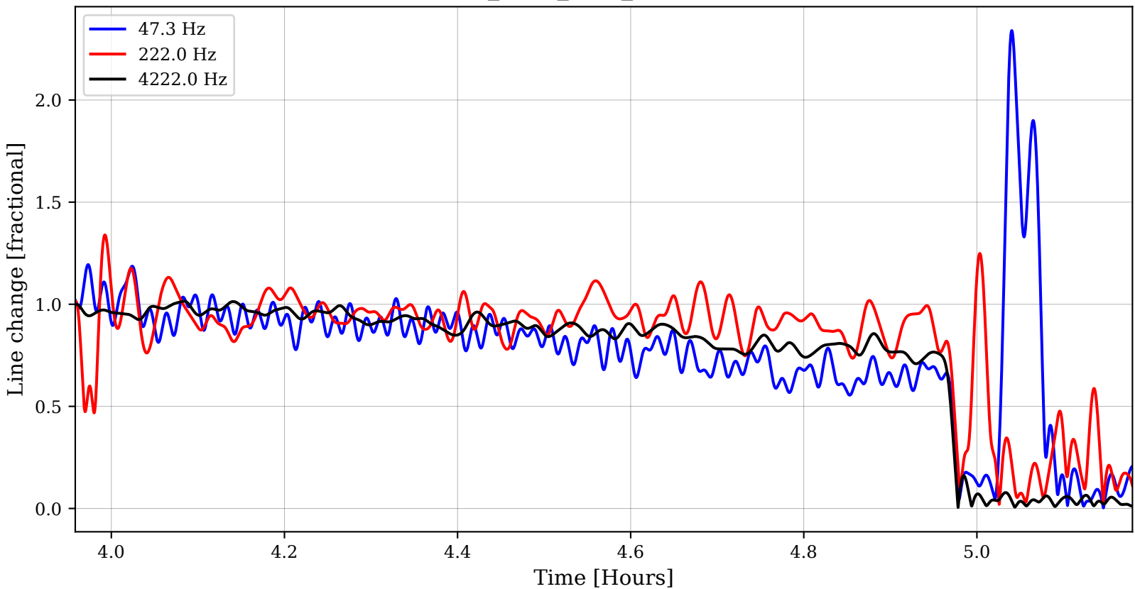
H1:OMC-DCPD_SUM_OUT_DQ Intensity injections
