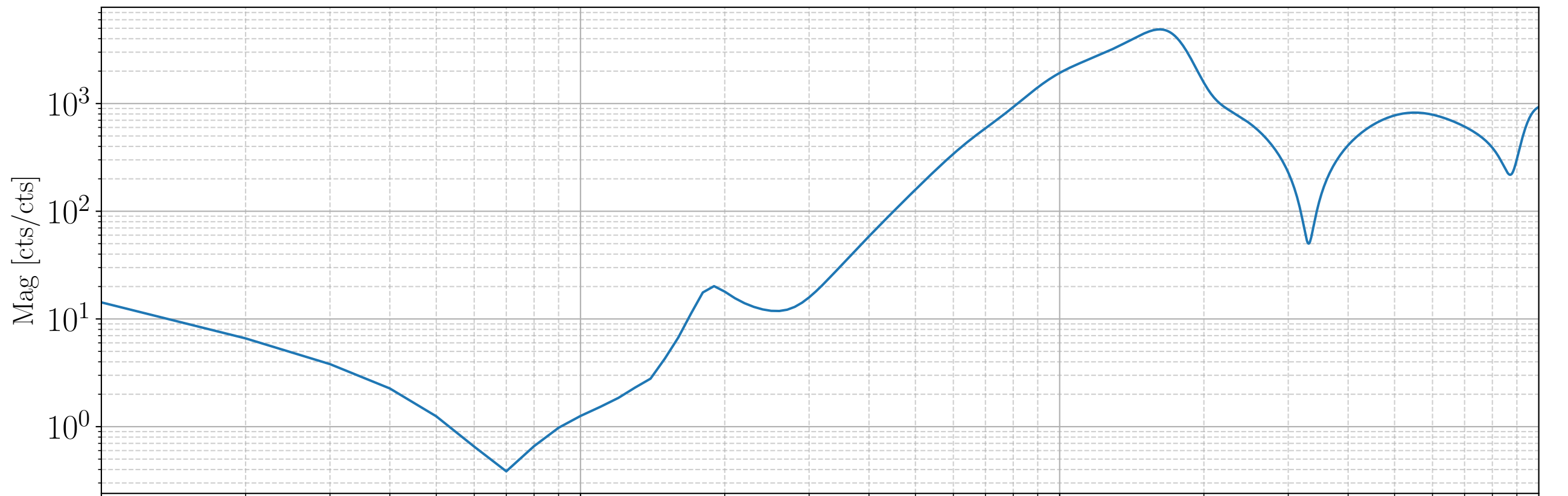
Sum of CHARD Y + RPC filter modules at 1359873048
