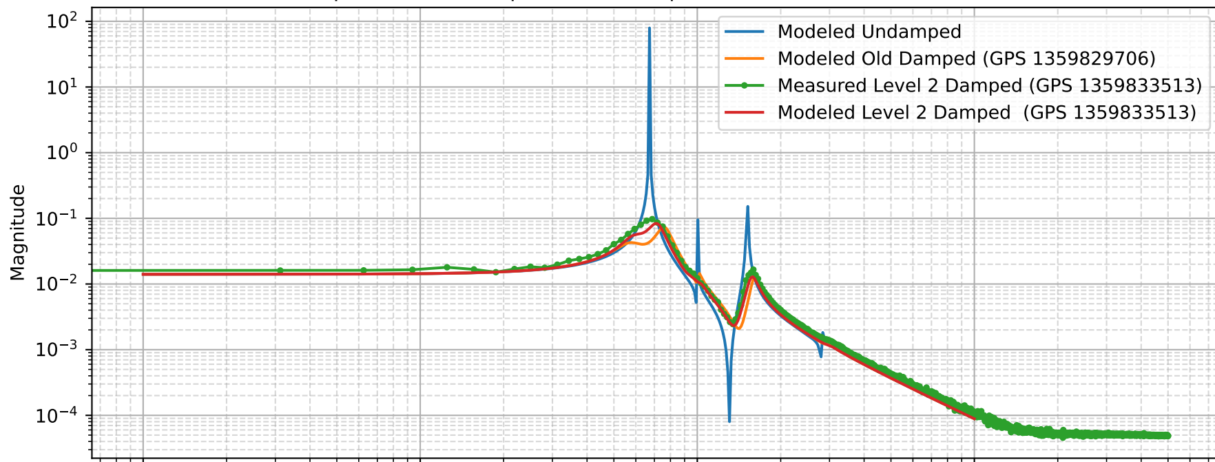
Level 2 Damped vs Old Damped vs Undamped SRM M3 L to M3 L transfer functions
