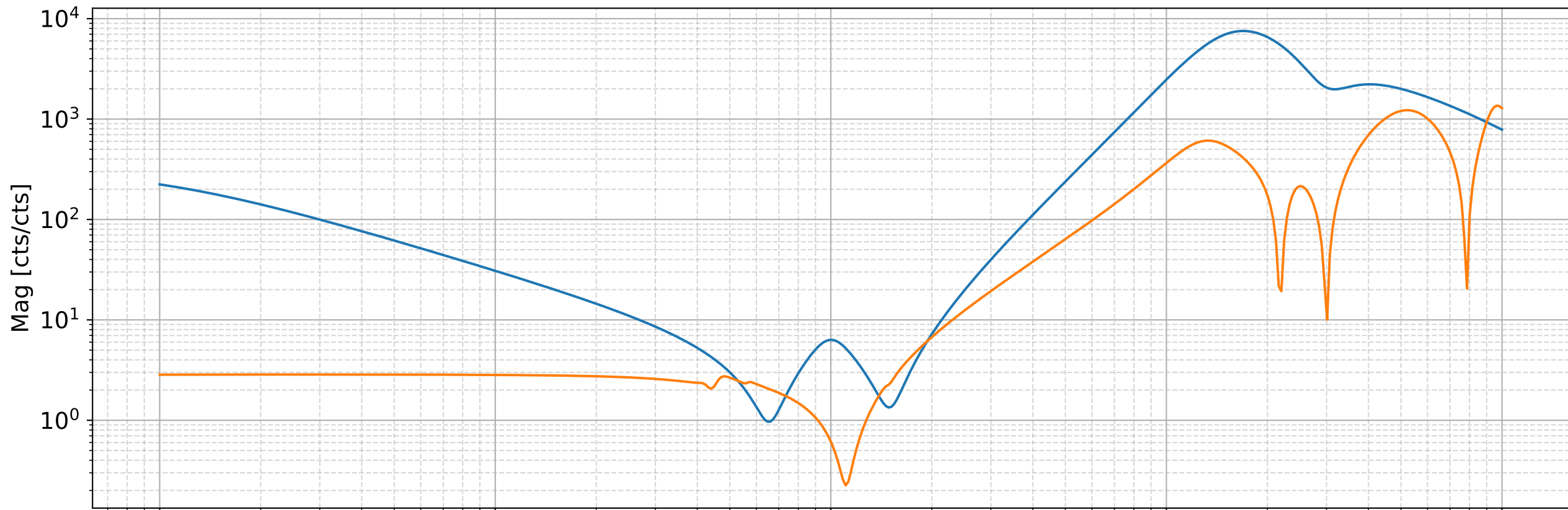
Raw ASC-DHARD P filter modules at 1360783399
