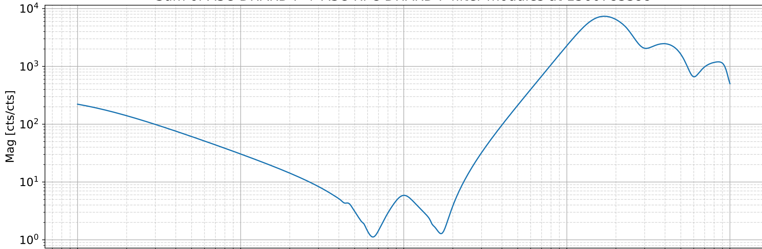
Sum of ASC-DHARD P + ASC-RPC DHARD P filter modules at 1360783399
