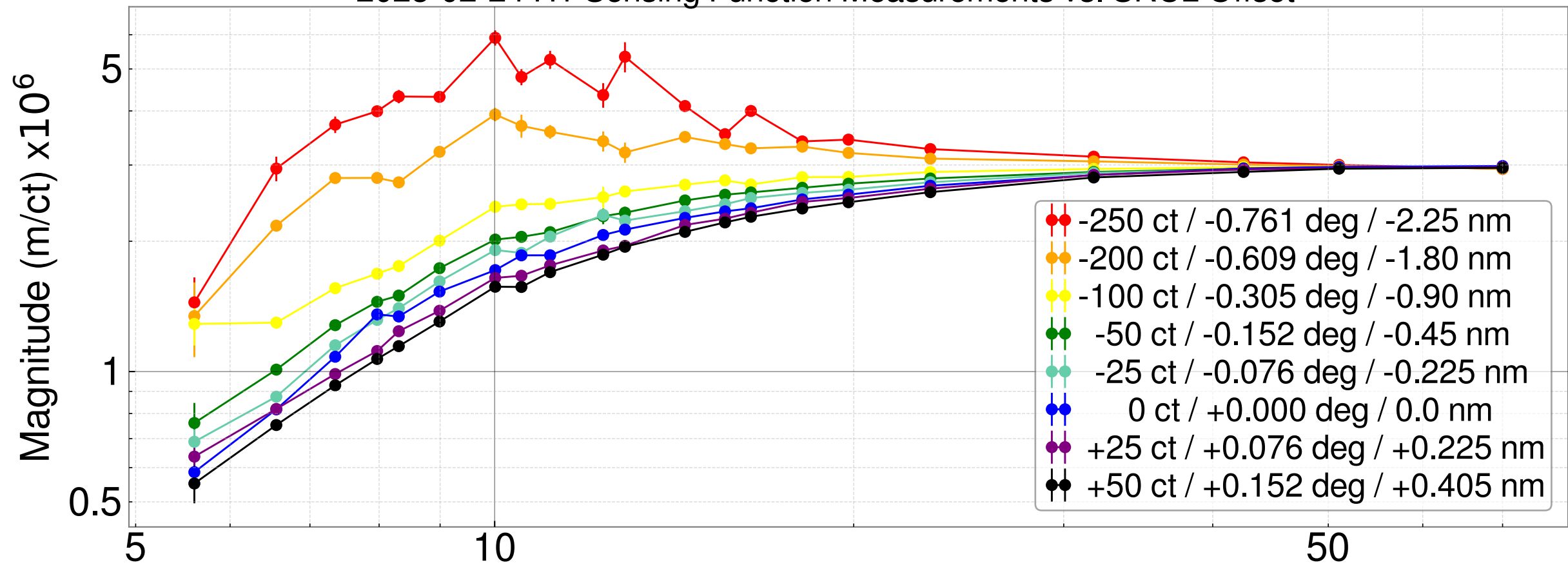
2023-02-24 H1 Sensing Function Measurements vs. SRCL Offset
