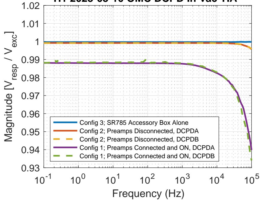
H1 2023-03-10 OMC DCPD In-vac TIA
