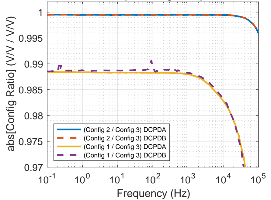
"Meas Setup" Config Comparison
