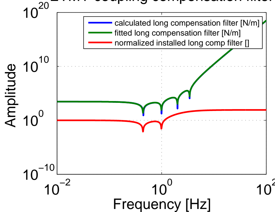
ETMY coupling compensation filter
