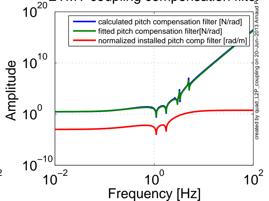
ETMY coupling compensation filter
