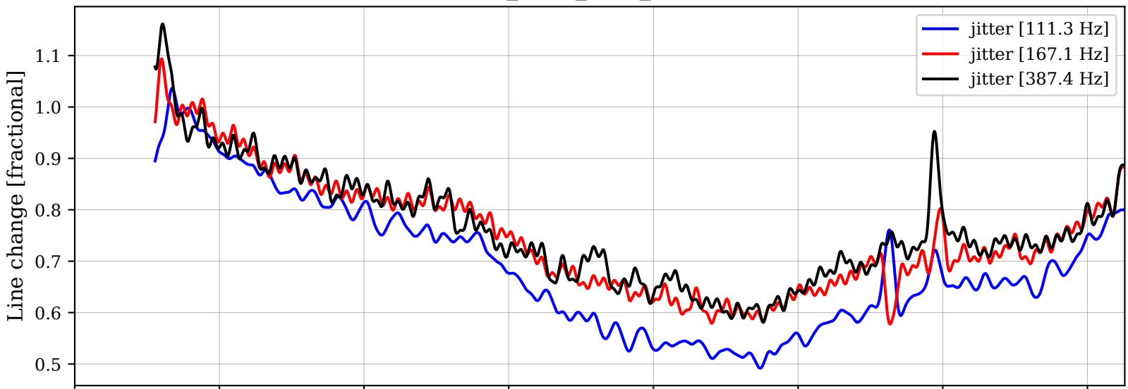
H1:OMC-DCPD_SUM_OUT_DQ jitter injections
