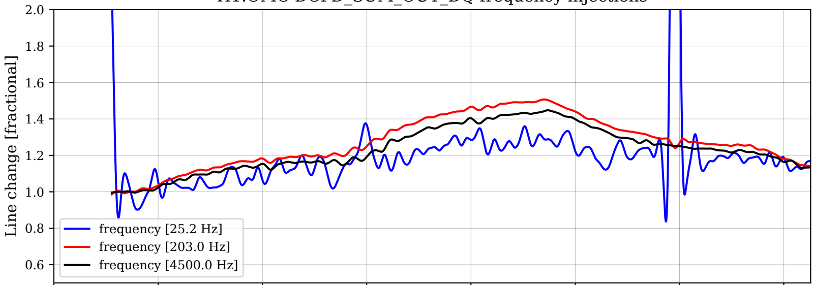
H1:OMC-DCPD_SUM_OUT_DQ frequency injections
