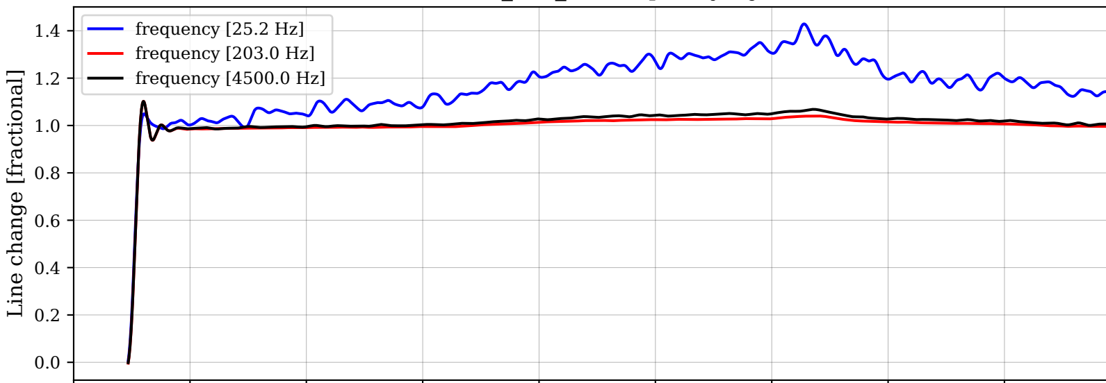
H1:LSC-PRCL_IN1_DQ frequency injections
