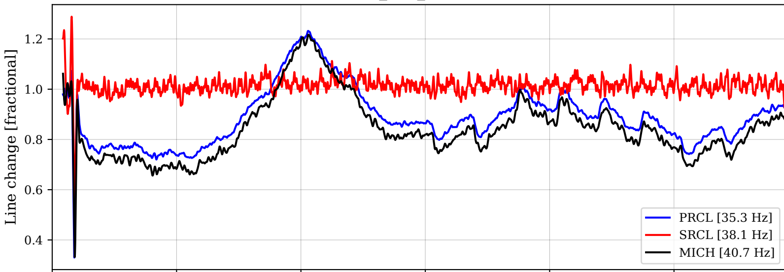
H1:LSC-SRCL_IN1_DQ LSC injections
