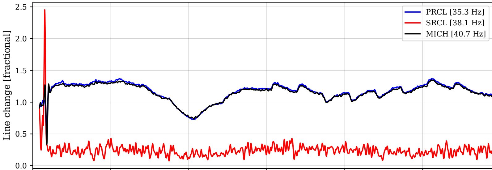
H1:LSC-PRCL_IN1_DQ LSC injections
