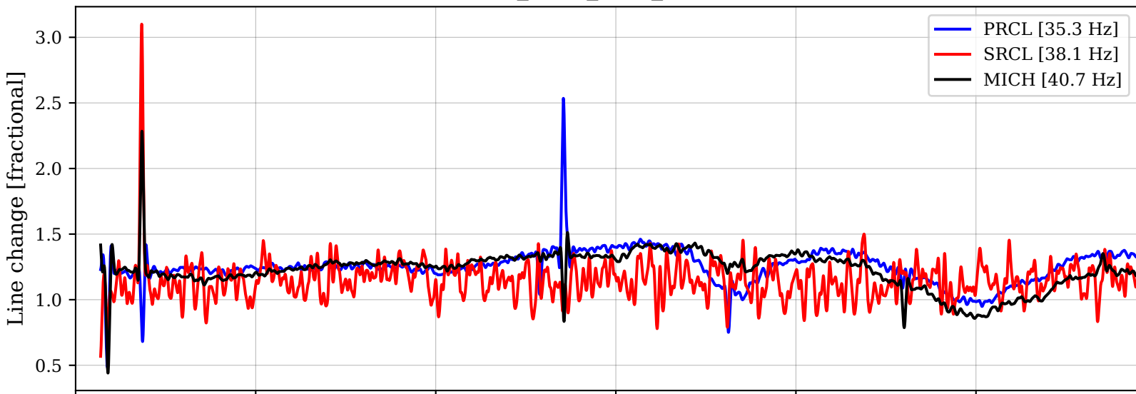
H1:OMC-DCPD_SUM_OUT_DQ LSC injections
