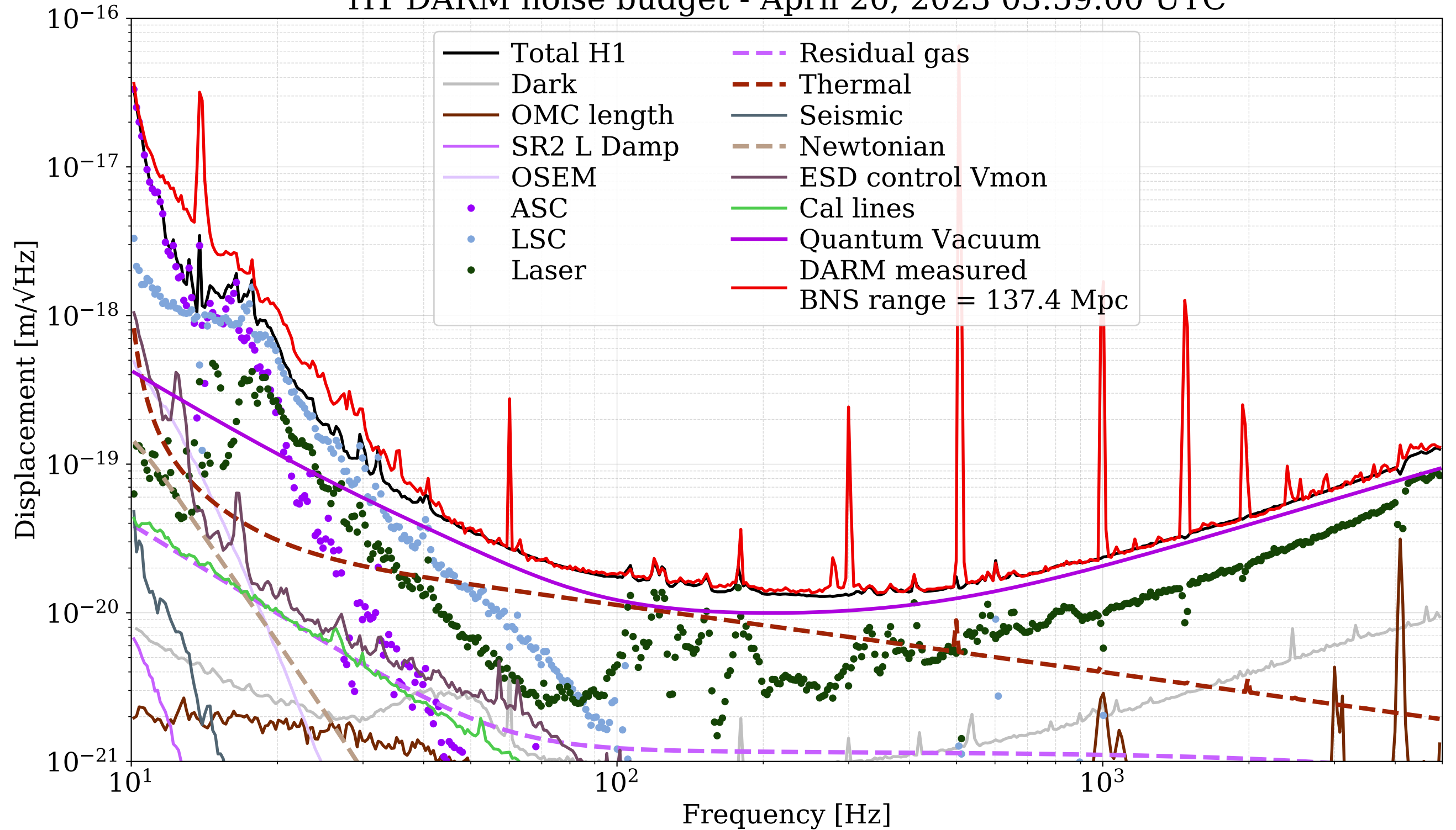
H1 DARM noise budget - April 20, 2023 03:59:00 UTC
