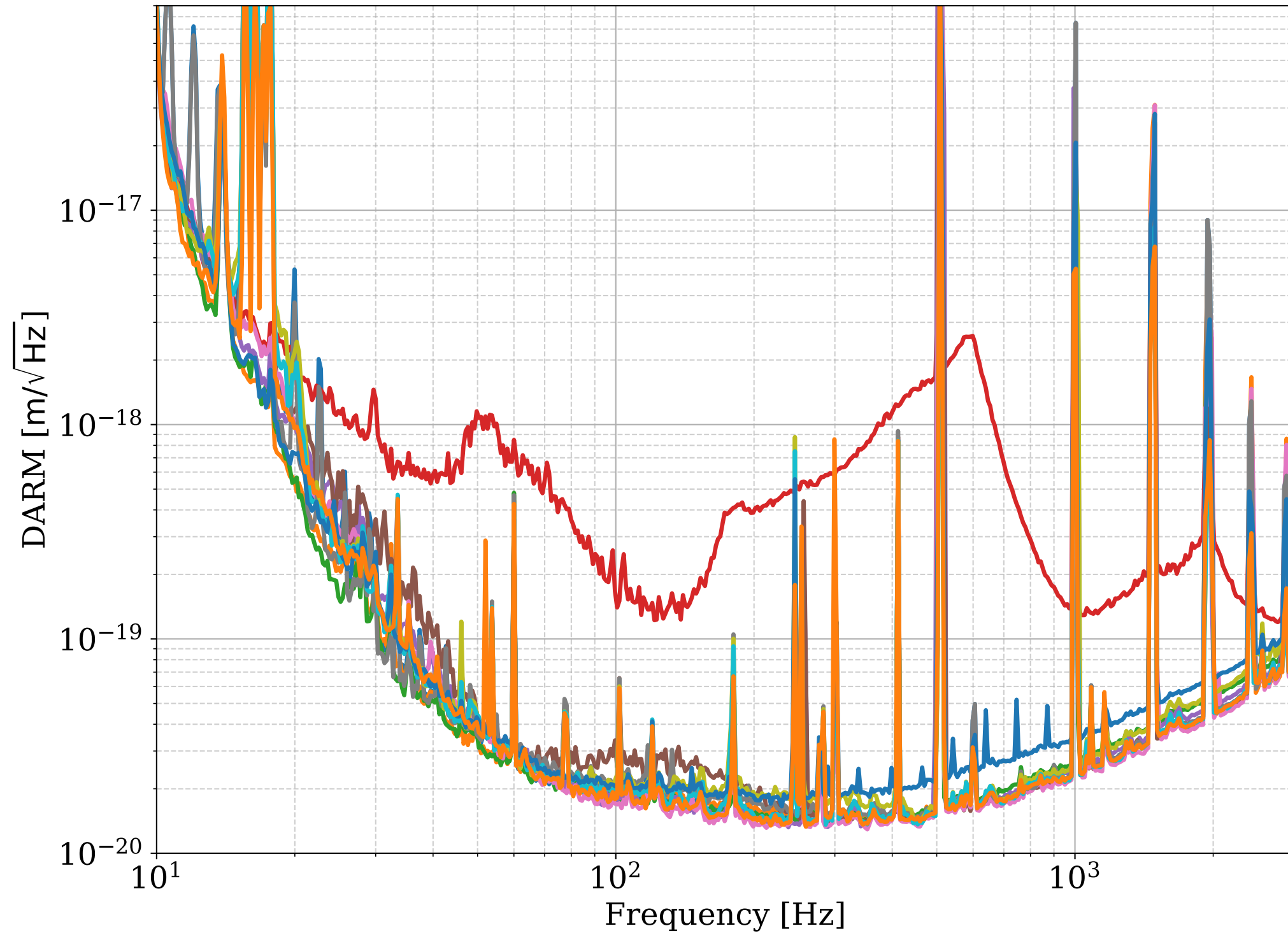
Pcal-corrected DARM
