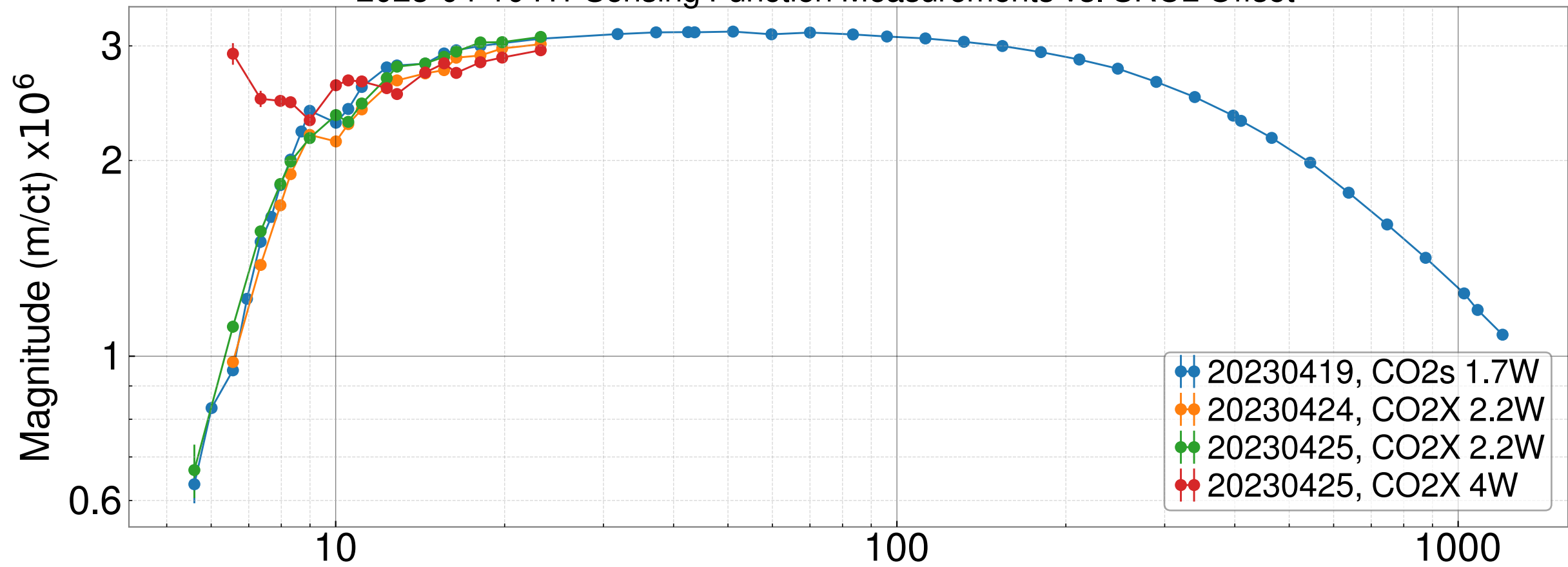
2023-04-10 H1 Sensing Function Measurements vs. SRCL Offset
