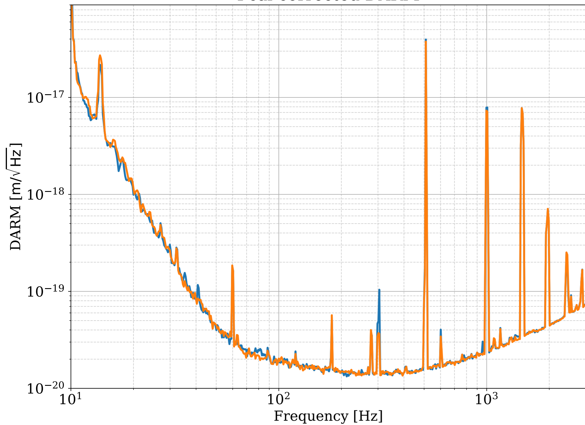
Pcal-corrected DARM
