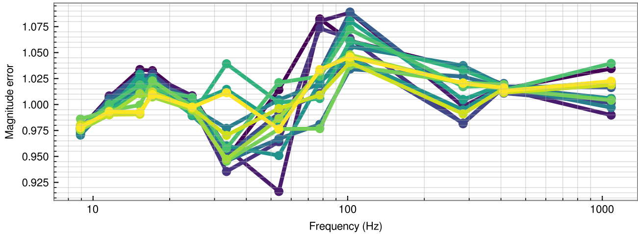
H1 response function evolution with time (blue=start of epoch; yellow=end of epoch) Measured response / reference response
