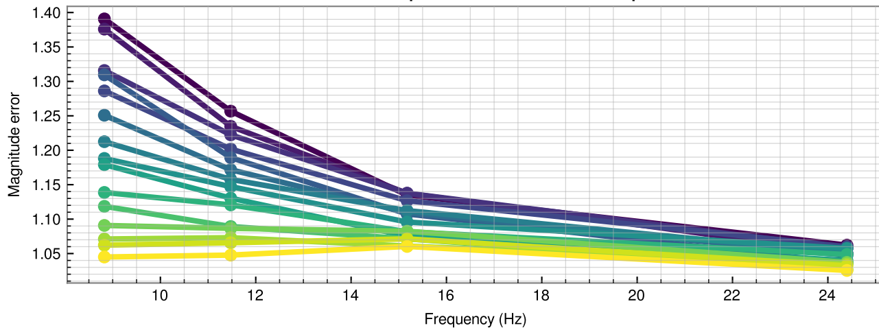
H1 sensing function evolution with time (blue=start of epoch; yellow=end of epoch) Measured response / nominal response
