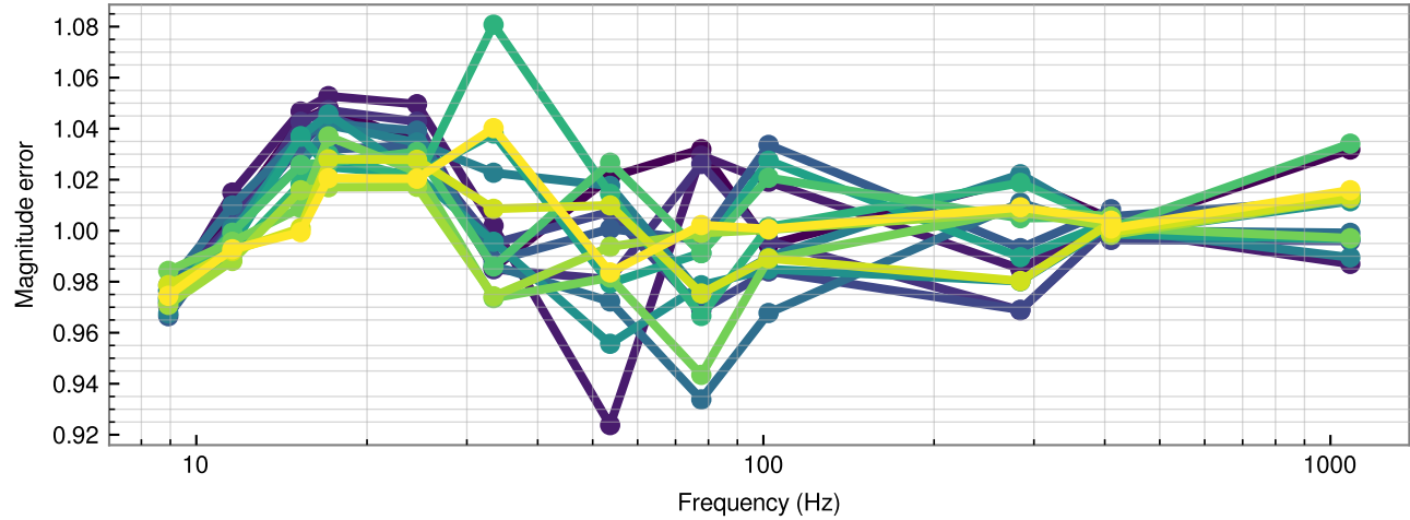
H1 response function evolution with time (blue=start of epoch; yellow=end of epoch) Measured response / nominal response
