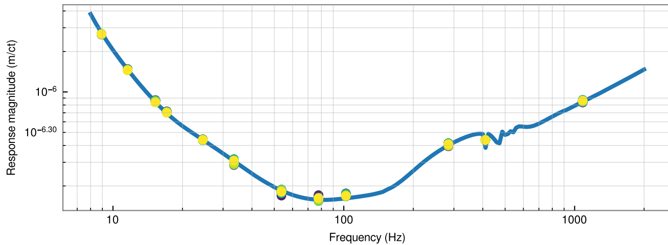
H1 response function evolution with time (blue=start of epoch; yellow=end of epoch)
