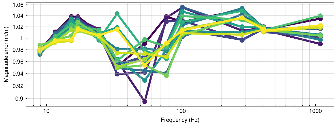
H1 systematic error evolution with time (blue=start of epoch; yellow=end of epoch)
