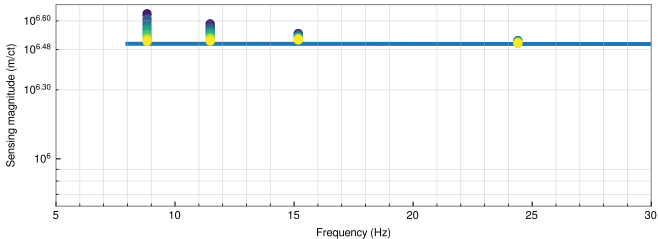
H1 sensing function evolution with time (blue=start of epoch; yellow=end of epoch)
