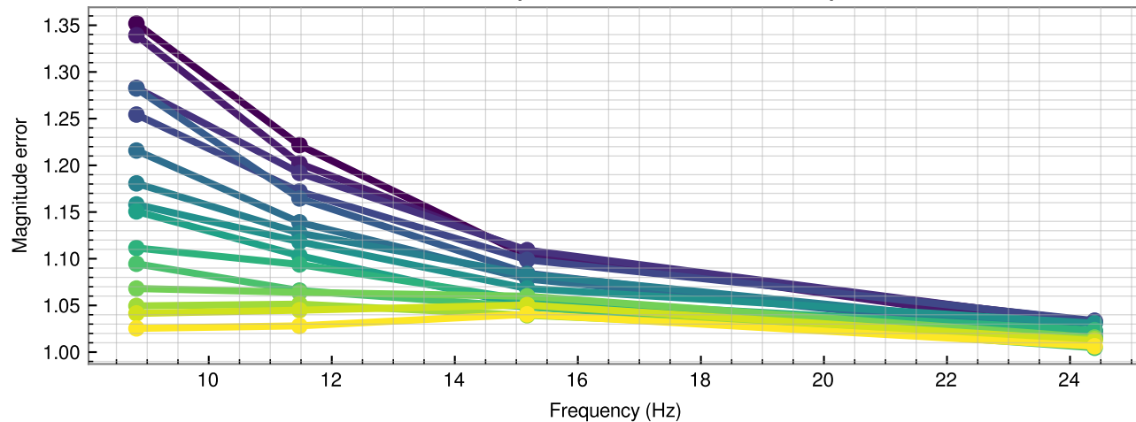
H1 sensing function evolution with time (blue=start of epoch; yellow=end of epoch) Measured response / reference response
