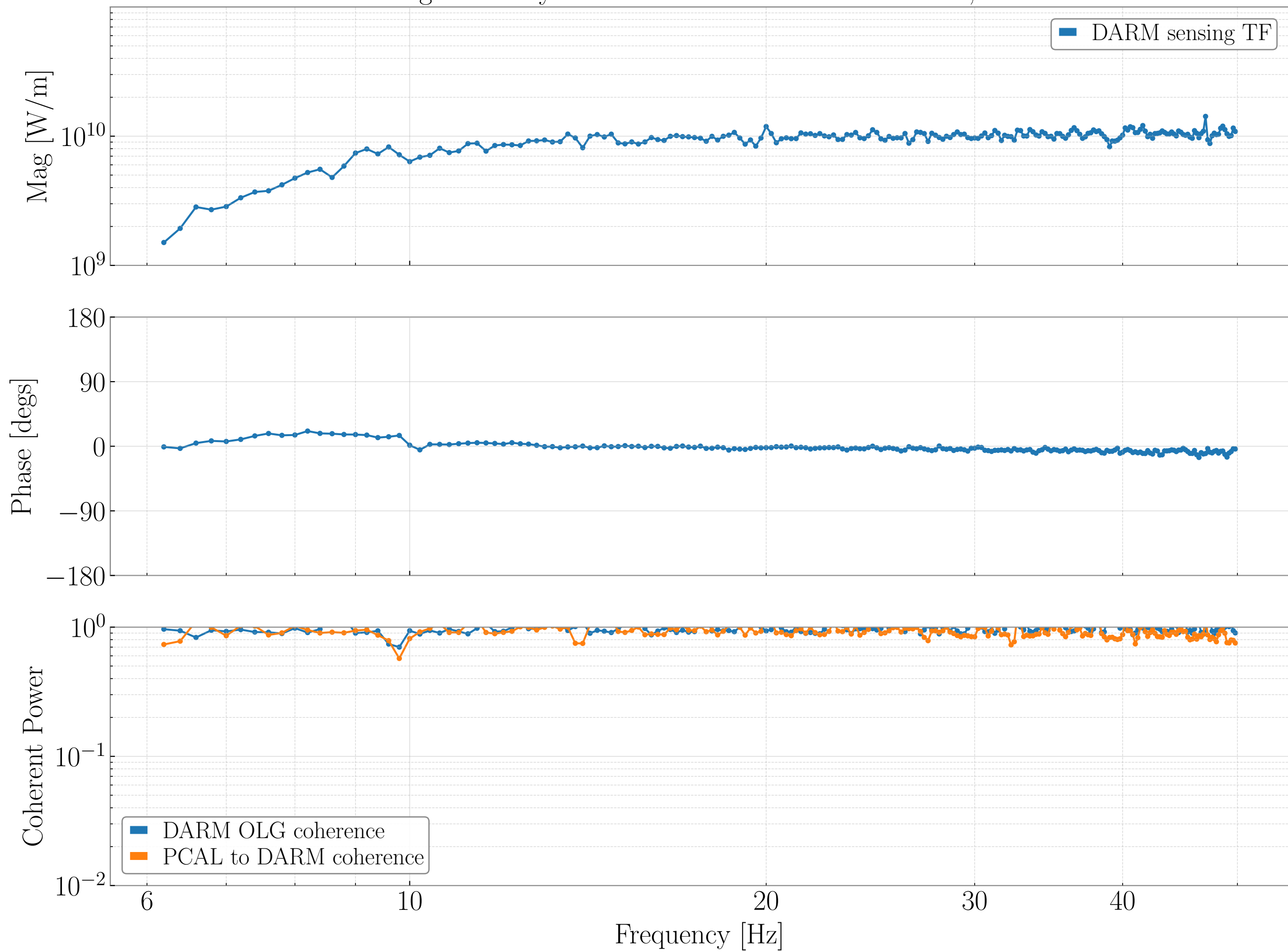
DARM Sensing TF - May 5th 2023 - SRCL offset counts - 200, 40mA DARM
