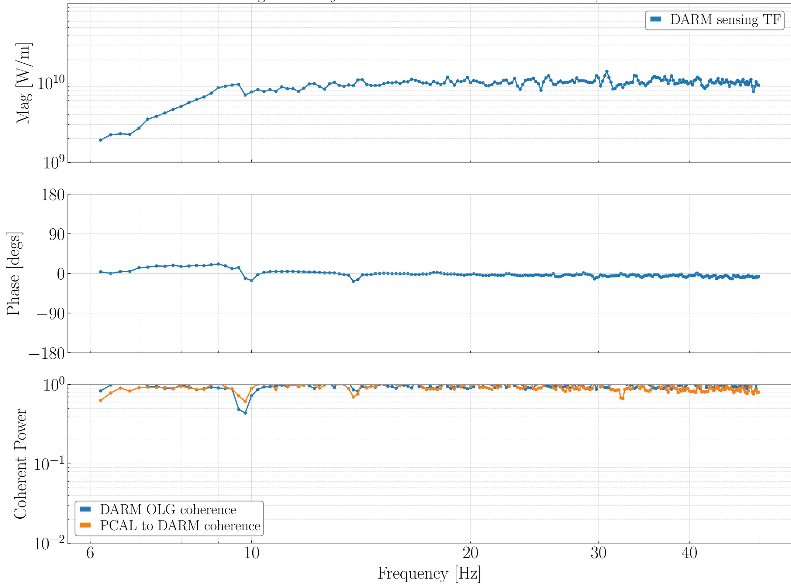
DARM Sensing TF - May 5th 2023 - SRCL offset counts - 220, 40mA DARM
