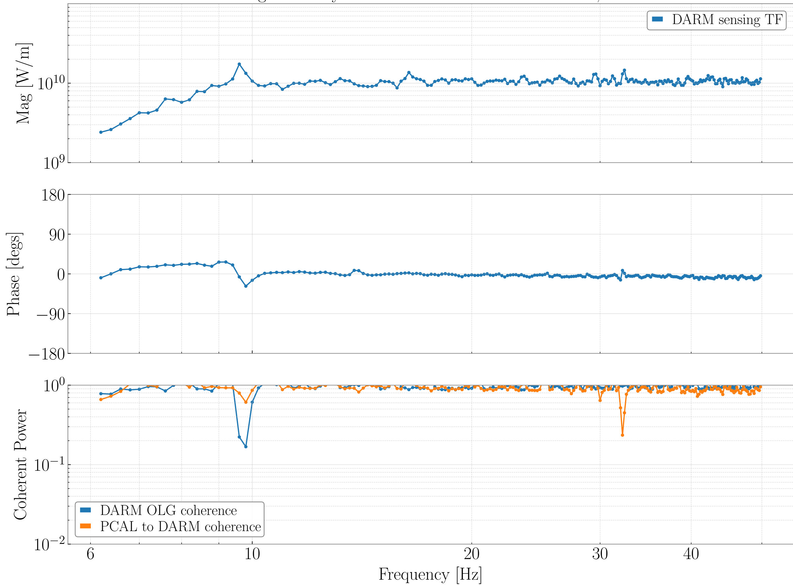
DARM Sensing TF - May 5th 2023 - SRCL offset counts - 265, 40mA DARM
