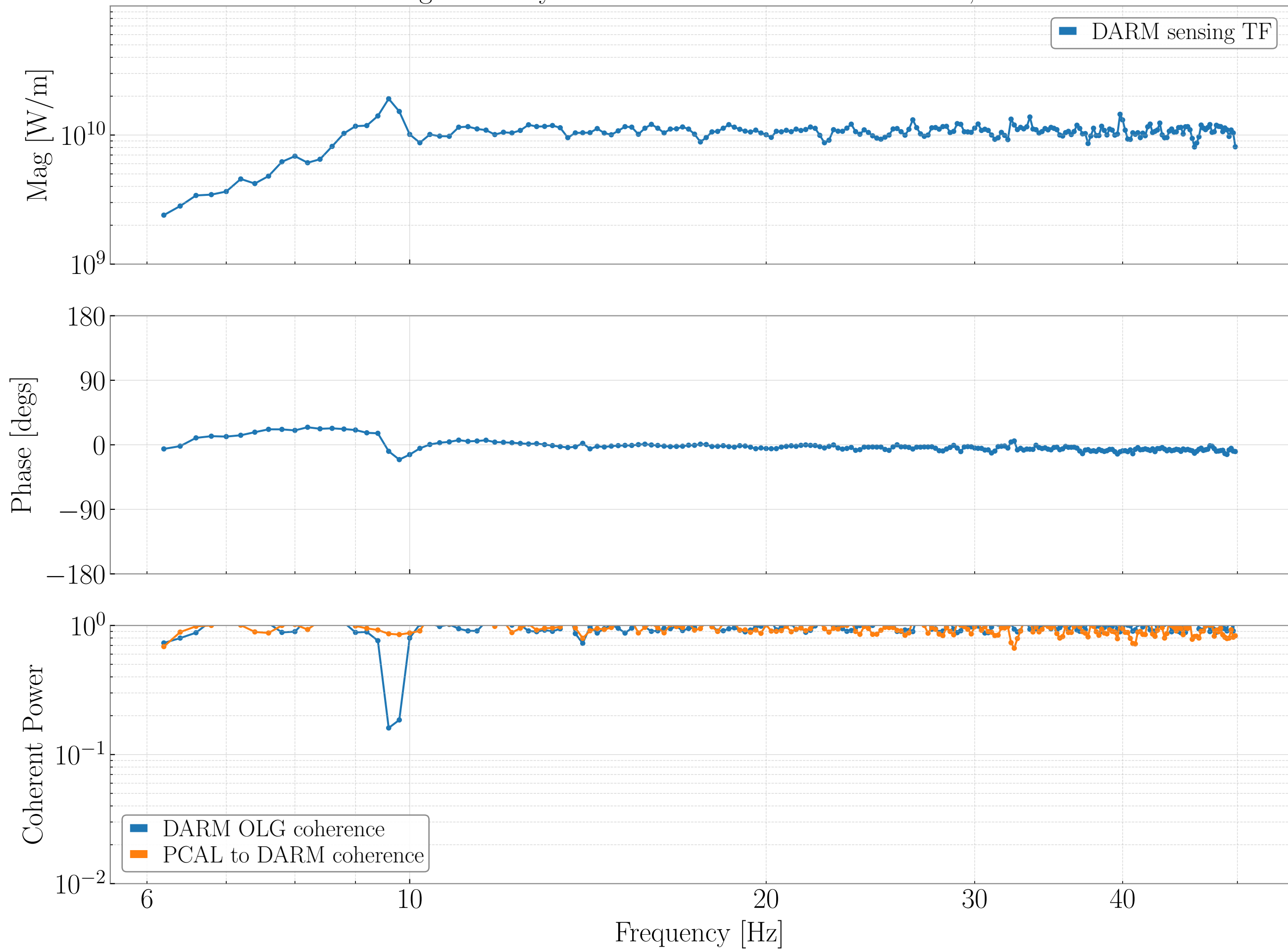
DARM Sensing TF - May 5th 2023 - SRCL offset counts - 275, 40mA DARM
