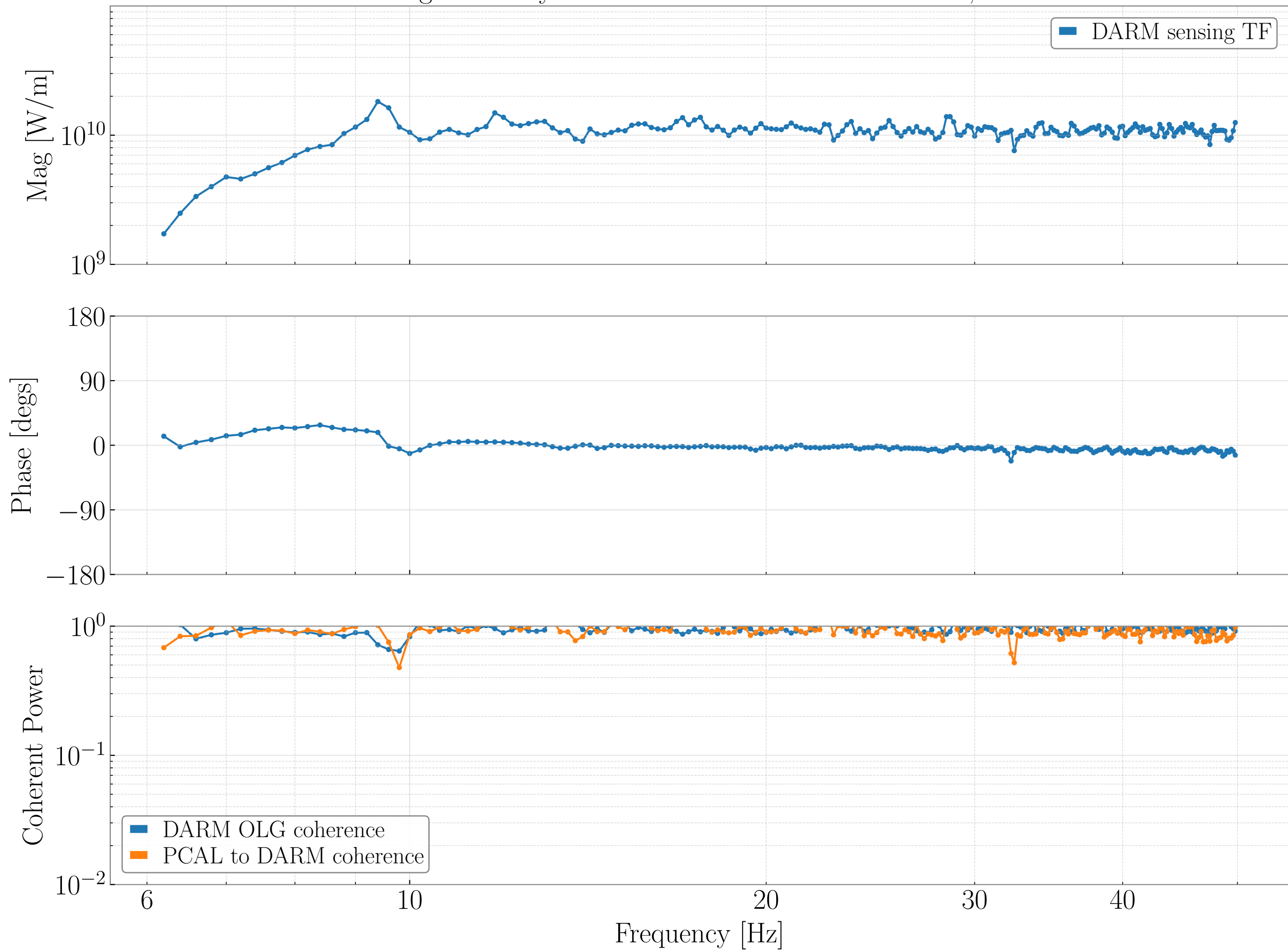
DARM Sensing TF - May 5th 2023 - SRCL offset counts - 290, 40mA DARM
