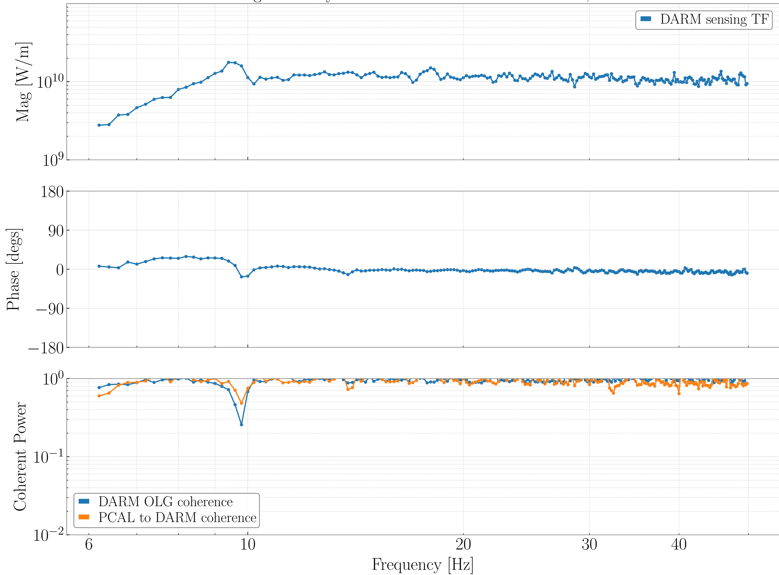
DARM Sensing TF - May 5th 2023 - SRCL offset counts - 300, 40mA DARM
