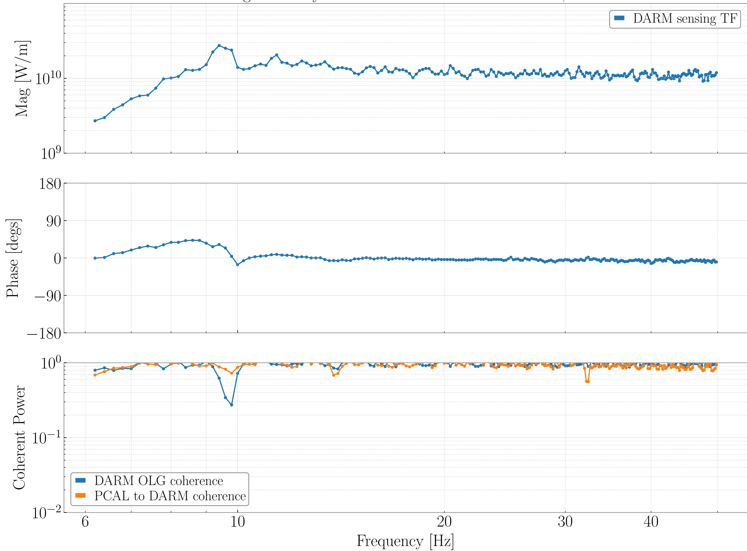
DARM Sensing TF - May 5th 2023 - SRCL offset counts - 350, 40mA DARM
