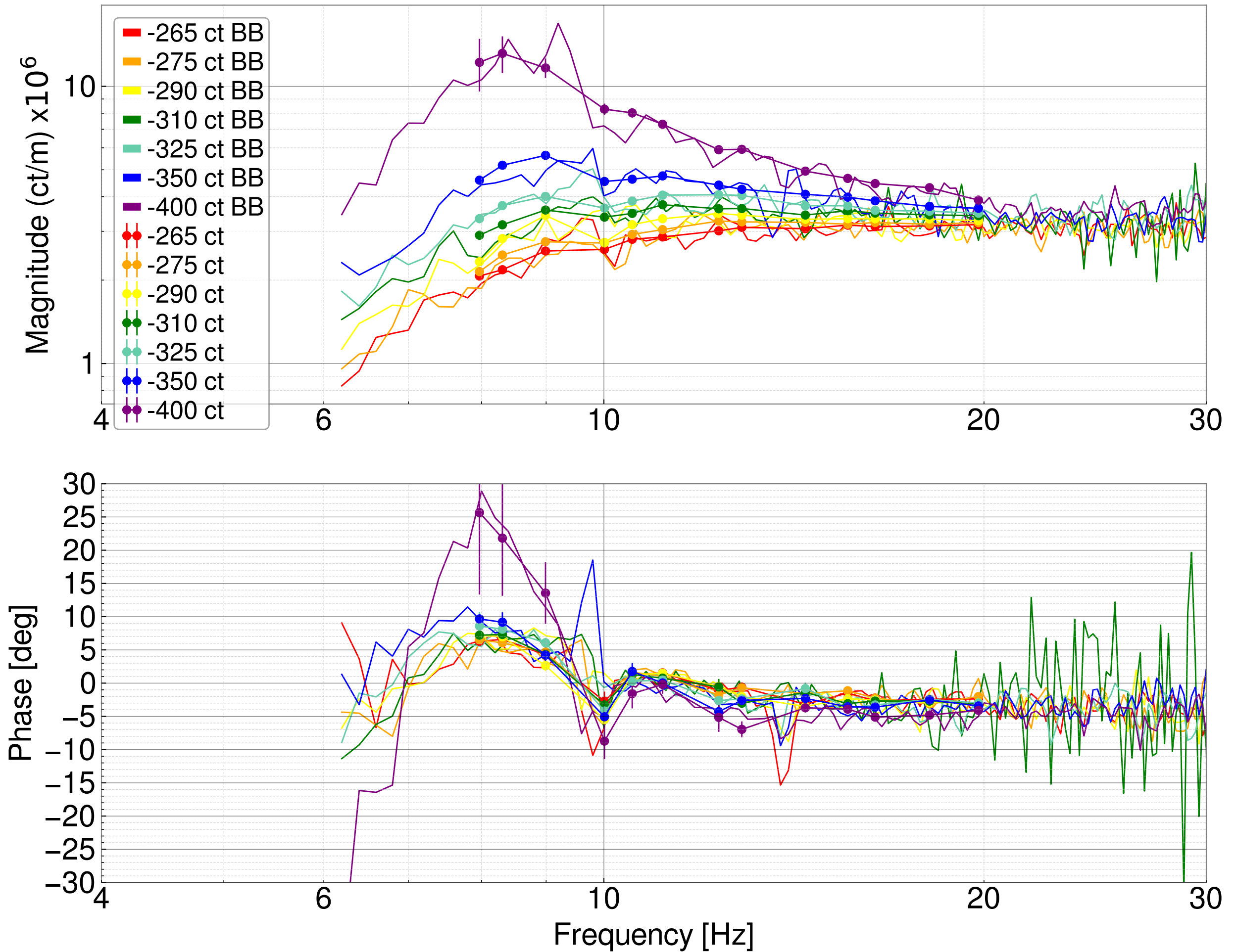
2023-05-08 H1 Sensing Function Measurements vs. SRCL Offset
