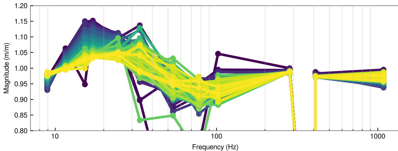
H1 Measured Systematic Error (PCAL / DELTA EXT) (blue = may 9 2023 01:15:00 UTC; yellow = may 9 2023 04:30:00 UTC)
