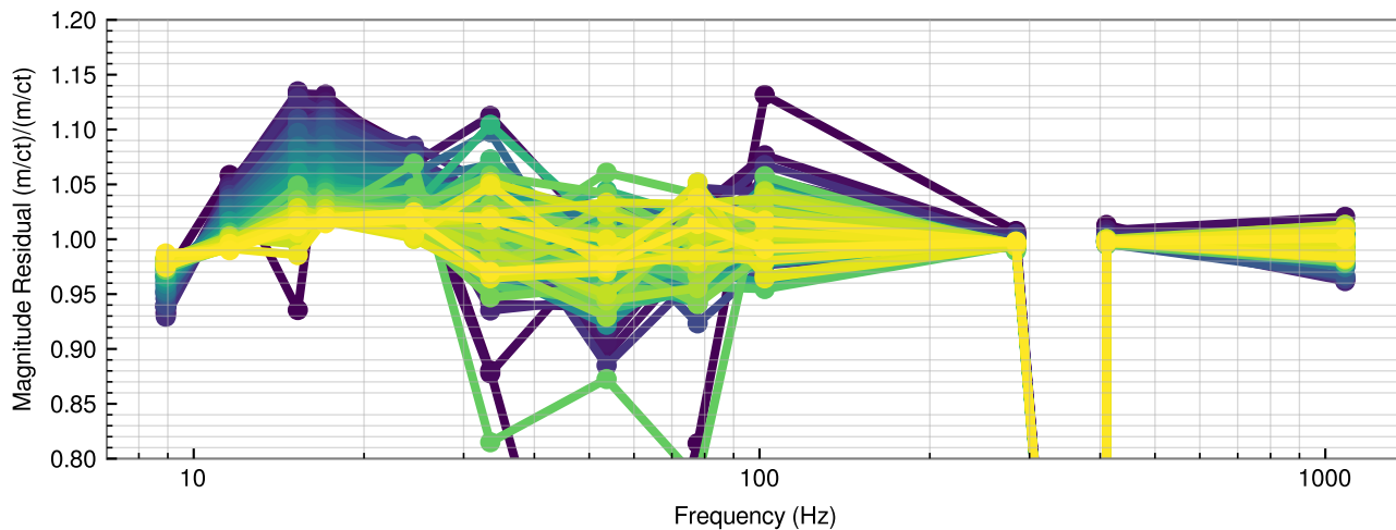
H1 Response Function Ratio: (PCAL/DARM ERR) / (Model w/o TDCFs) (blue = may 9 2023 01:15:00 UTC; yellow = may 9 2023 04:30:00 UTC)
