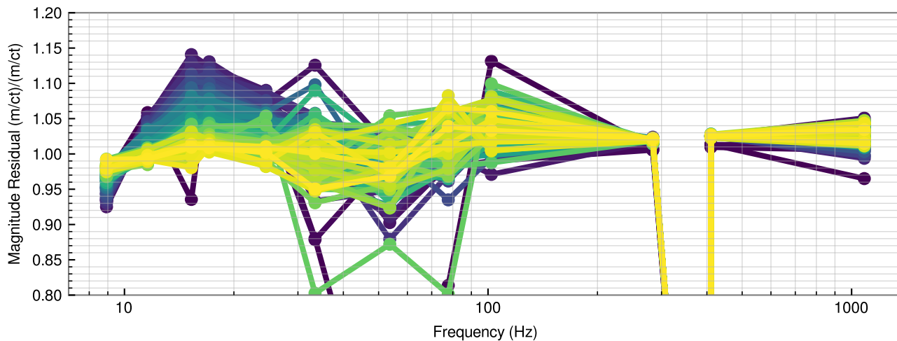
H1 Response Function Ratio: (PCAL/DARM ERR) / (Model w/ TDCFs) (blue = may 9 2023 01:15:00 UTC; yellow = may 9 2023 04:30:00 UTC)
