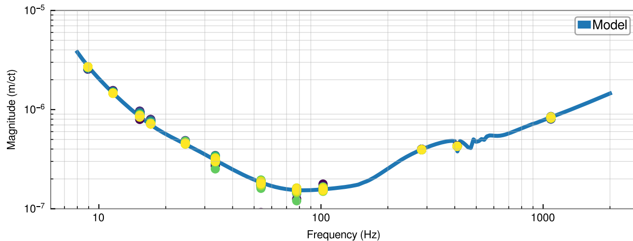
H1 Response Function Time Evolution (1+G)/C (blue = may 9 2023 01:15:00 UTC; yellow = may 9 2023 04:30:00 UTC)
