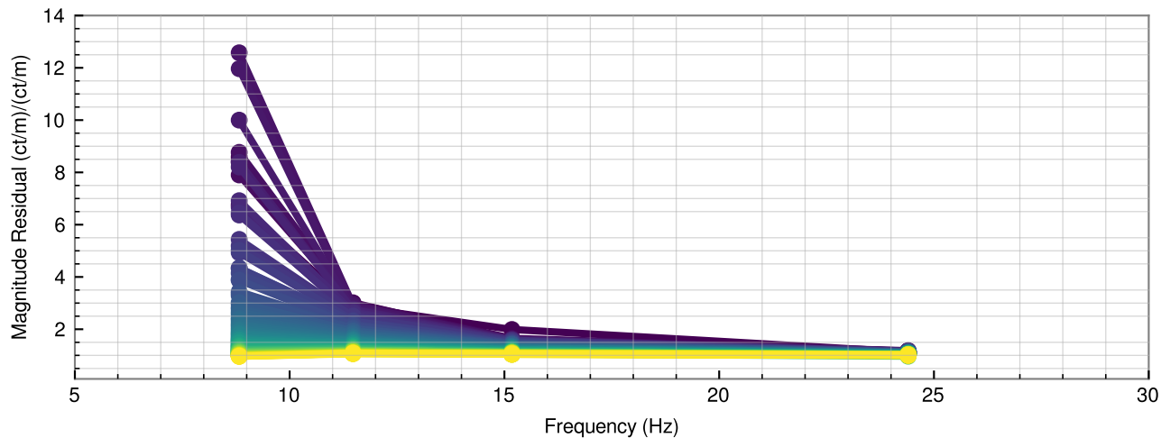
H1 Sensing Function Ratio: Meas / (Model w/ TDCFs) (blue = may 9 2023 01:15:00 UTC; yellow = may 9 2023 04:30:00 UTC)
