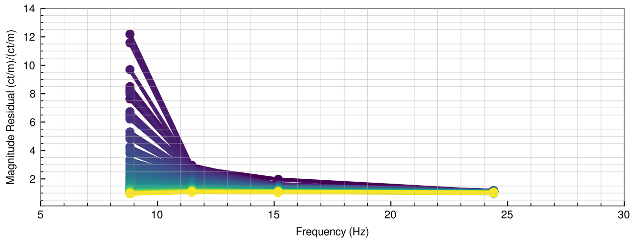
H1 Sensing Function Ratio: Meas / (Model w/o TDCFs) (blue = may 9 2023 01:15:00 UTC; yellow = may 9 2023 04:30:00 UTC)
