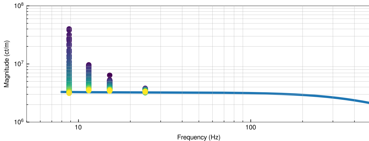
H1 Sensing Function: Meas vs. (Model w/o TDCFs) (blue = may 9 2023 01:15:00 UTC; yellow = may 9 2023 04:30:00 UTC)
