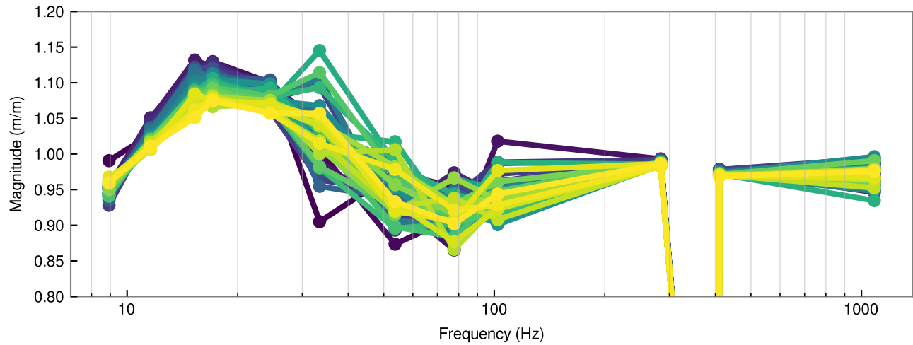
H1 Measured Systematic Error (PCAL / DELTAL EXT) (blue = may 10 2023 08:41:00 UTC; yellow = may 10 2023 10:12:00 UTC)
