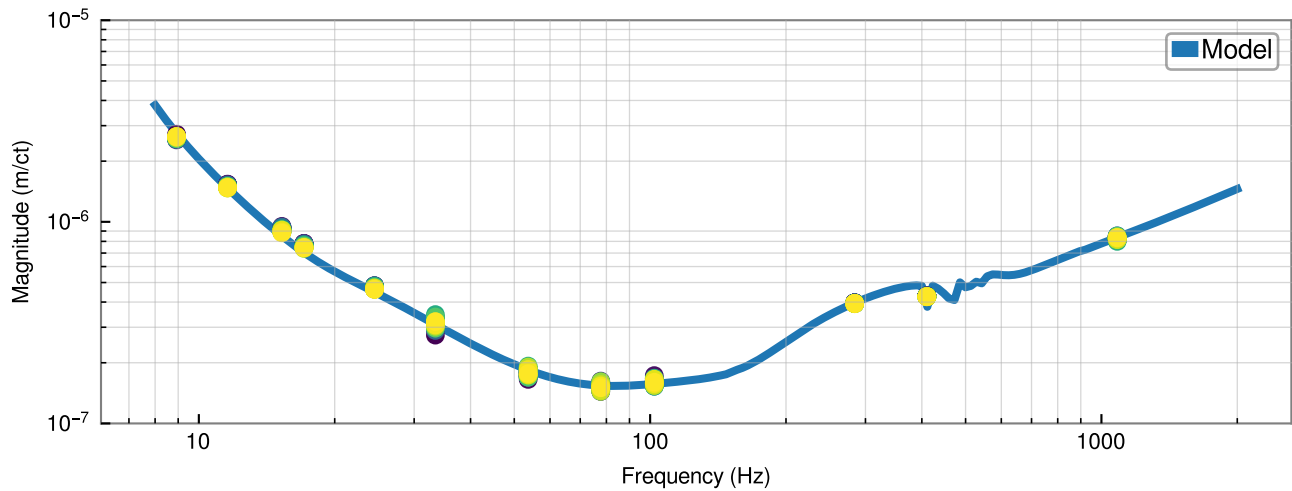
H1 Response Function Time Evolution (1+G)/C (blue = may 10 2023 08:41:00 UTC; yellow = may 10 2023 10:12:00 UTC)
