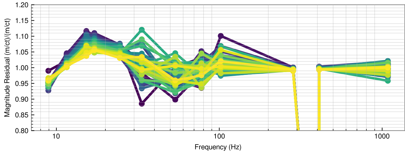
H1 Response Function Ratio: (PCAL/DARM ERR) / (Model w/o TDCFs) (blue = may 10 2023 08:41:00 UTC; yellow = may 10 2023 10:12:00 UTC)
