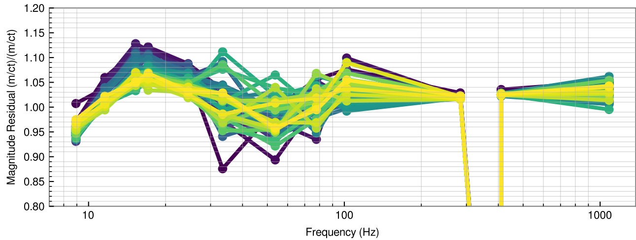
H1 Response Function Ratio: (PCAL/DARM ERR) / (Model w/ TDCFs) (blue = may 10 2023 08:41:00 UTC; yellow = may 10 2023 10:12:00 UTC)
