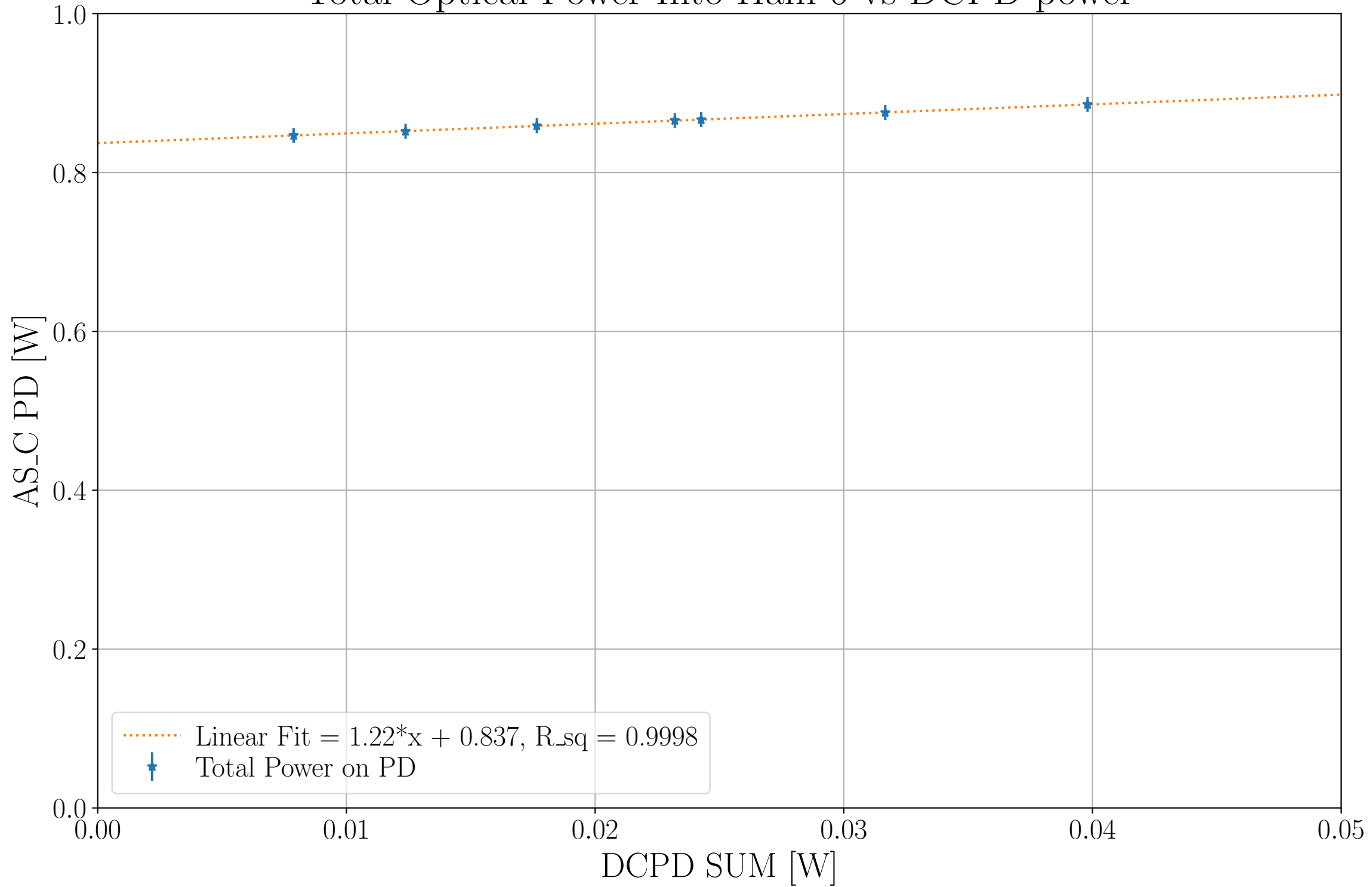
Total Optical Power Into Ham 6 vs DCPD power
