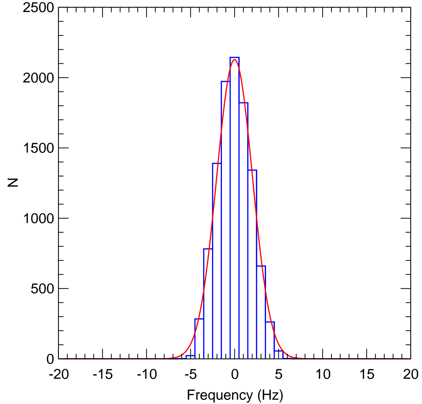
Histogram
