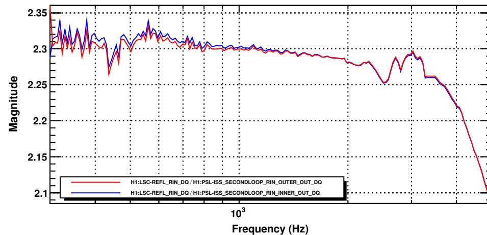
Transfer function (ifo total power reflection coefficient 7.32%, when thermalized: ~8.5%)
