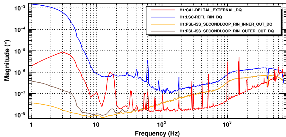
Power spectrum (INNER: 56.8mA, OUTER: 61.6mA, REFL: 9.0+9.0mW)
