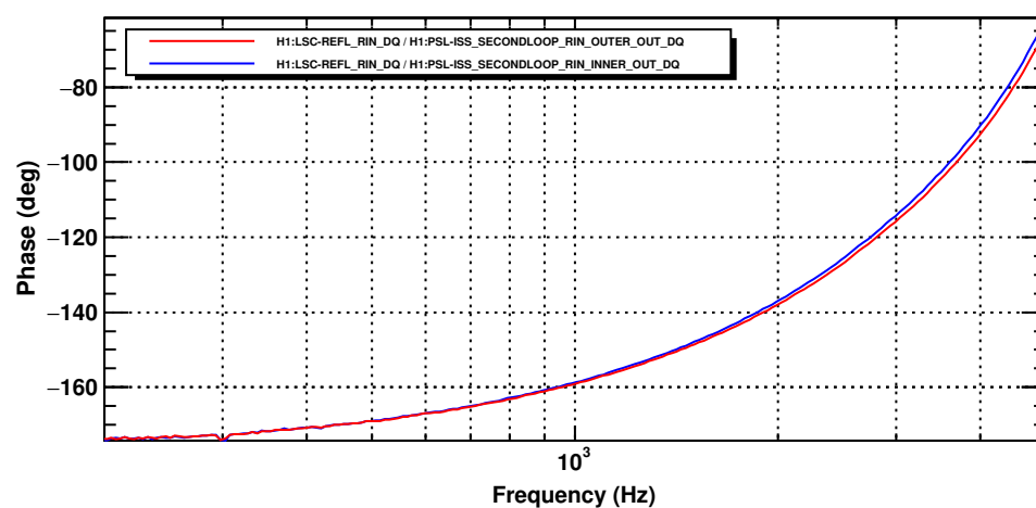
Transfer function
