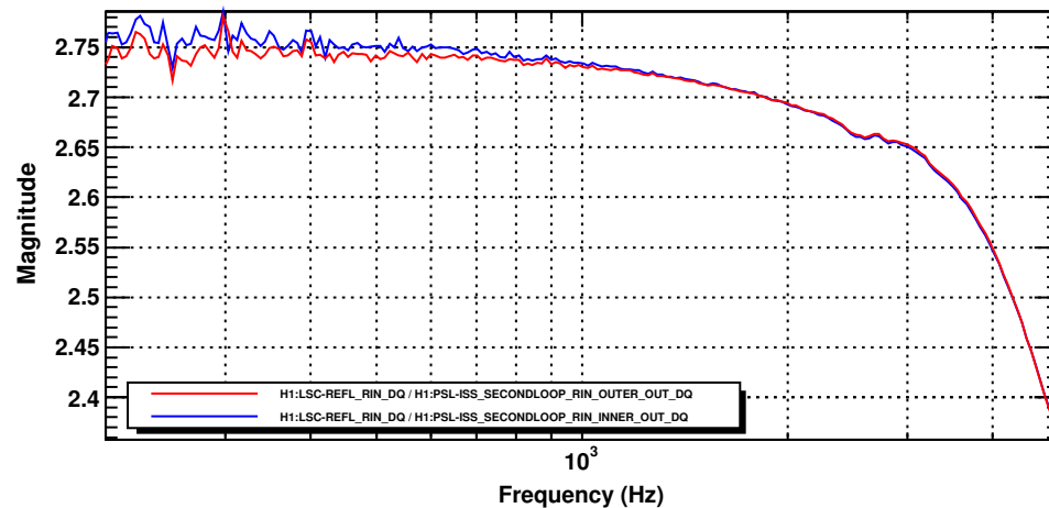
Transfer function (ifo total power reflection coefficient 6.86%)
