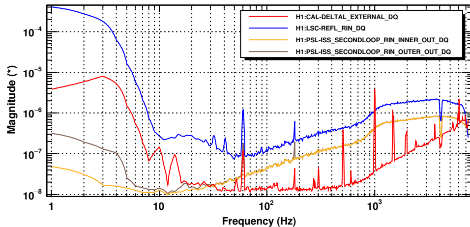
Power spectrum (INNER: 45.5mA, OUTER:49.3mA, REFL: 6.74+6.76mW)
