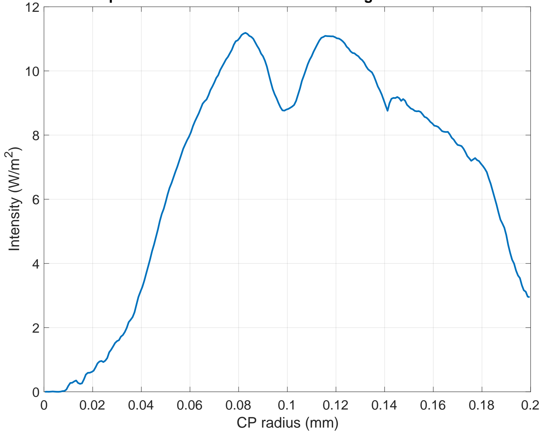
Fitted radial intensity - LHO aLOG 65832 Spatial scale estimated from HWS image: aLOG 65436
