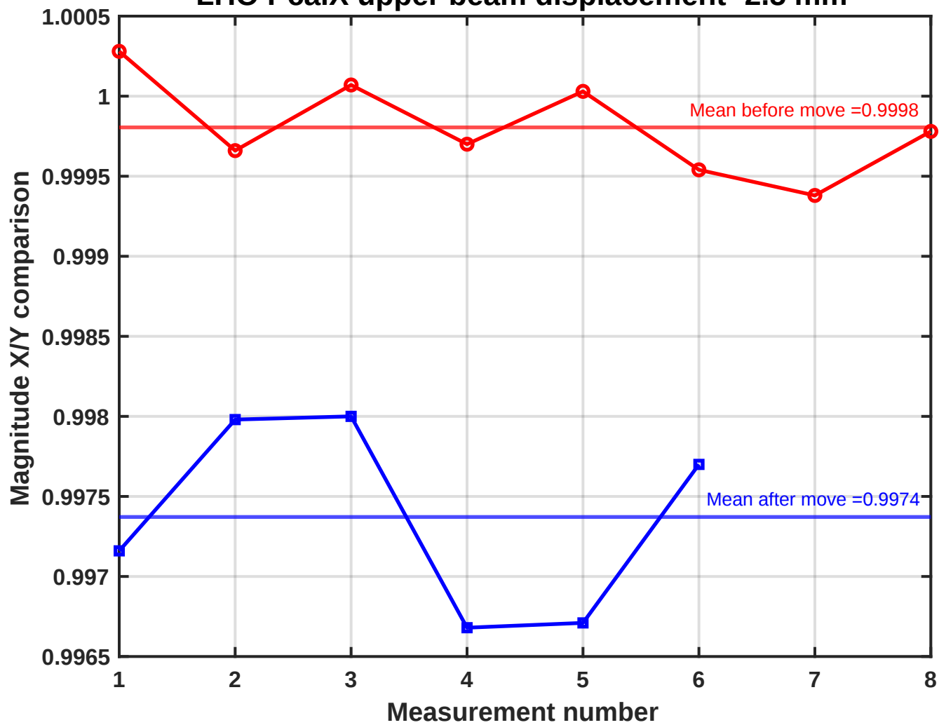
LHO PcalX upper beam displacement -2.5 mm
