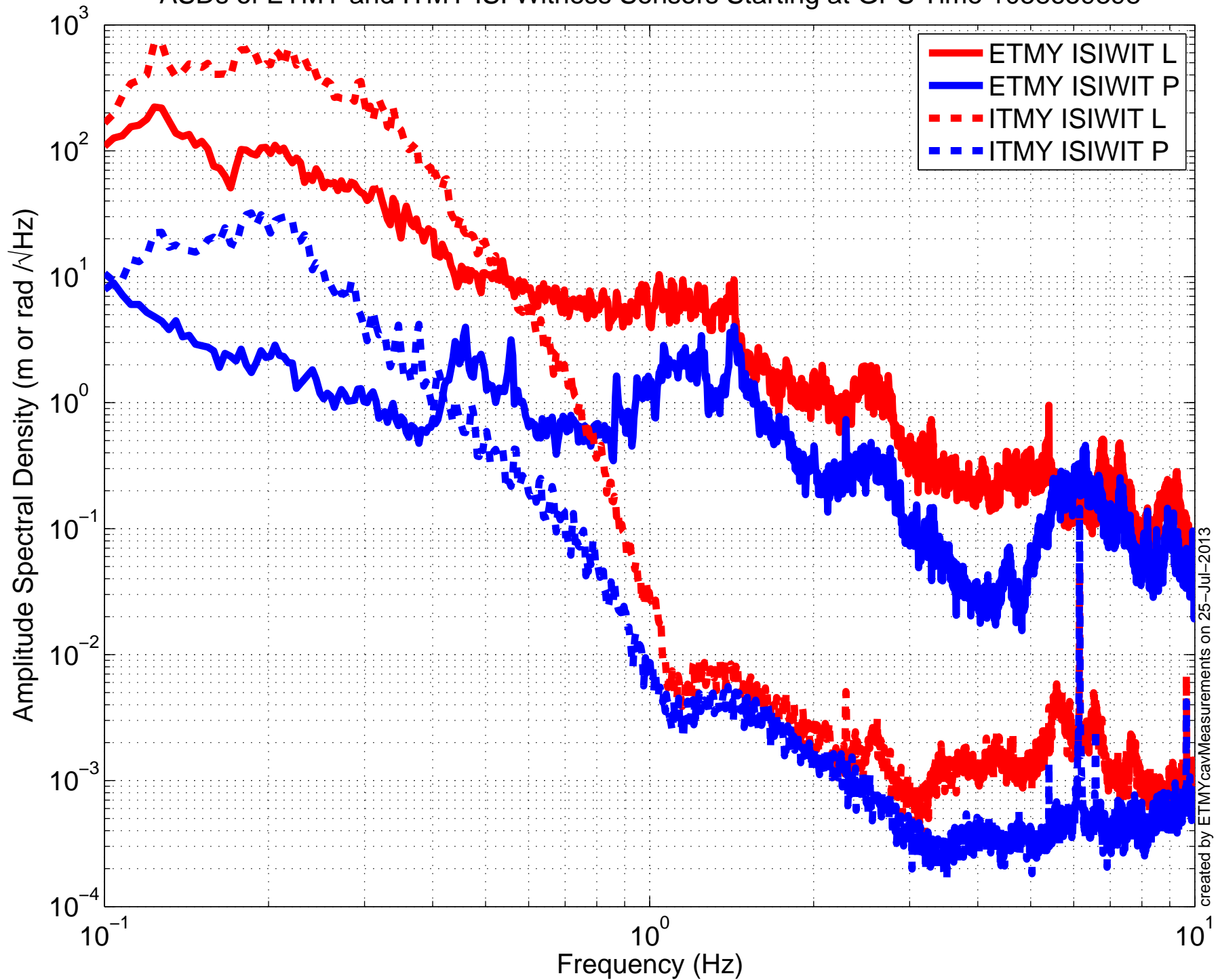
ASDs of ETMY and ITMY ISI Witness Sensors Starting at GPS Time 1058659398
