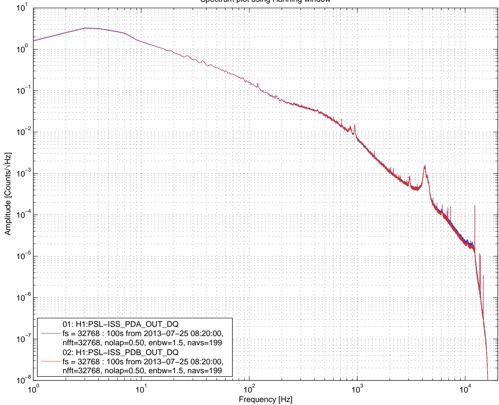
Spectrum plot using Hanning window
