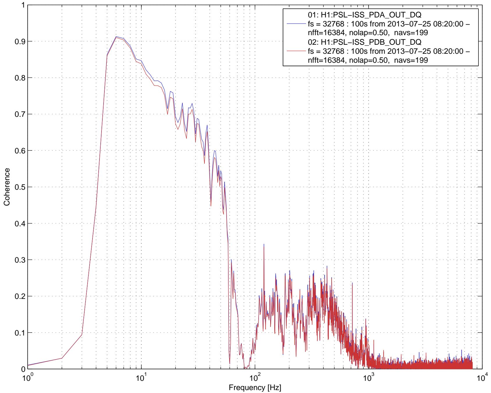
Coherence plot using Hanning window 03: H1:LSC-CARM_IN1_DQ fs = 16384 : 100s from 2013-07-25 08:20:00 -
