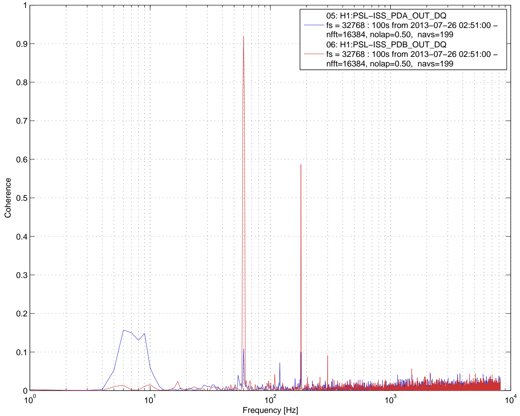
Coherence plot using Hanning window 04: H1:LSC-CARM_IN1_DQ fs = 16384 : 100s from 2013-07-26 02:51:00 -
