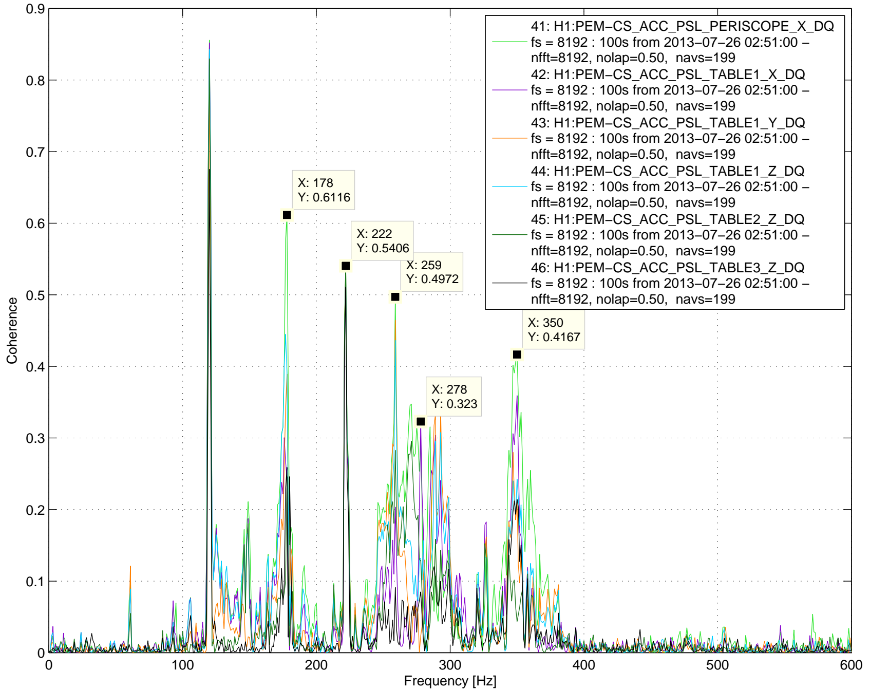
Coherence plot using Hanning window 30: H1:LSC-CARM_IN1_DQ fs = 16384 : 100s from 2013-07-26 02:51:00 -
