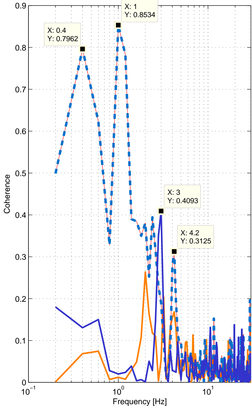
Coherence plot using Hanning window 01: H1:LSC-CARM_IN1_DQ fs = 16384 : 100s from 2013-07-26 02:51:00 -
