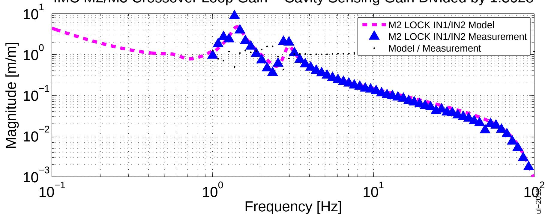
IMC M2/M3 Crossover Loop Gain – Cavity Sensing Gain Divided by 1.3628
