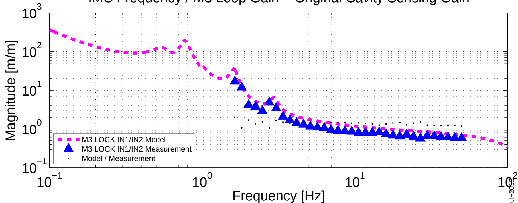
IMC Frequency / M3 Loop Gain – Original Cavity Sensing Gain
