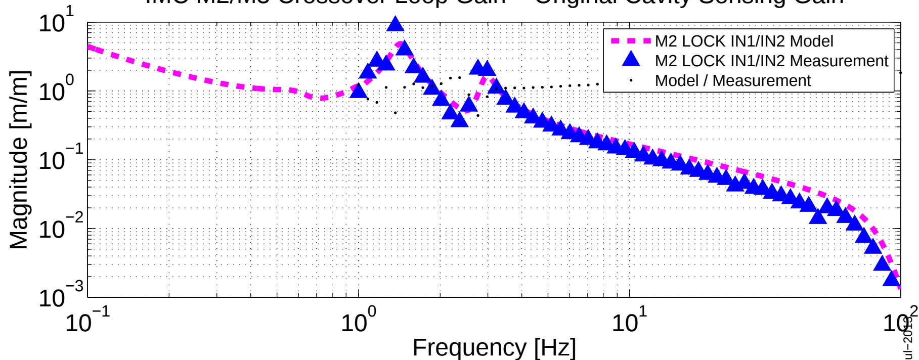
IMC M2/M3 Crossover Loop Gain – Original Cavity Sensing Gain
