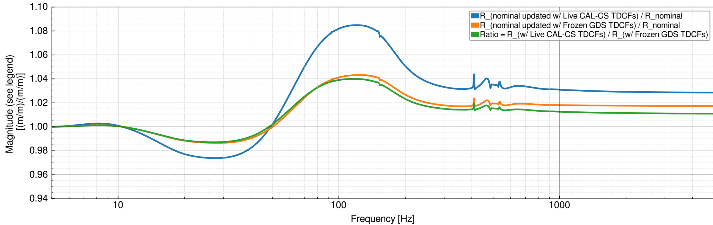
Systematic Error from using Frozen GDS TDCF vs. Live CAL-CS Values at 2023-07-26 01:10 UTC
