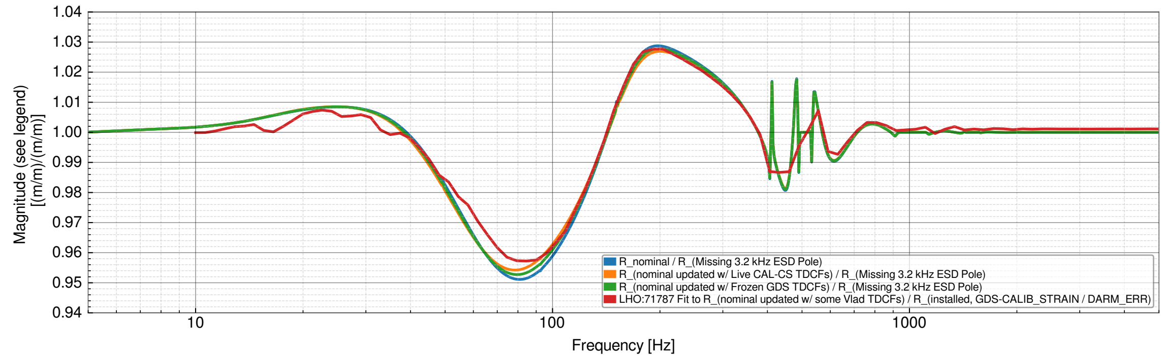
Systematic Error in R updated with Frozen GDS TDCF vs. Live CAL-CS Values at 2023-07-26 01:10 UTC, if missing 3.2 kHz ESD pole LHO:72622; NOT THERMALIZED
