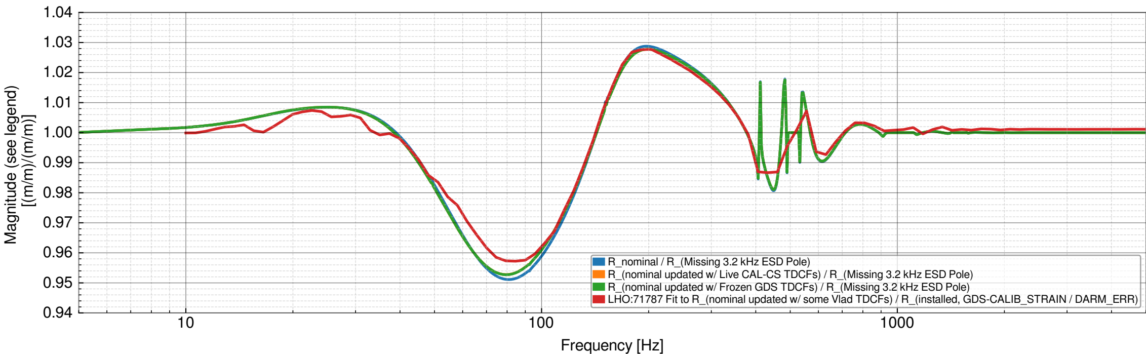
Systematic Error in R updated with Frozen GDS TDCF vs. Live CAL-CS Values at 2023-07-27 05:03:20 UTC, if missing 3.2 kHz ESD pole LHO:71787; THERMALIZED
