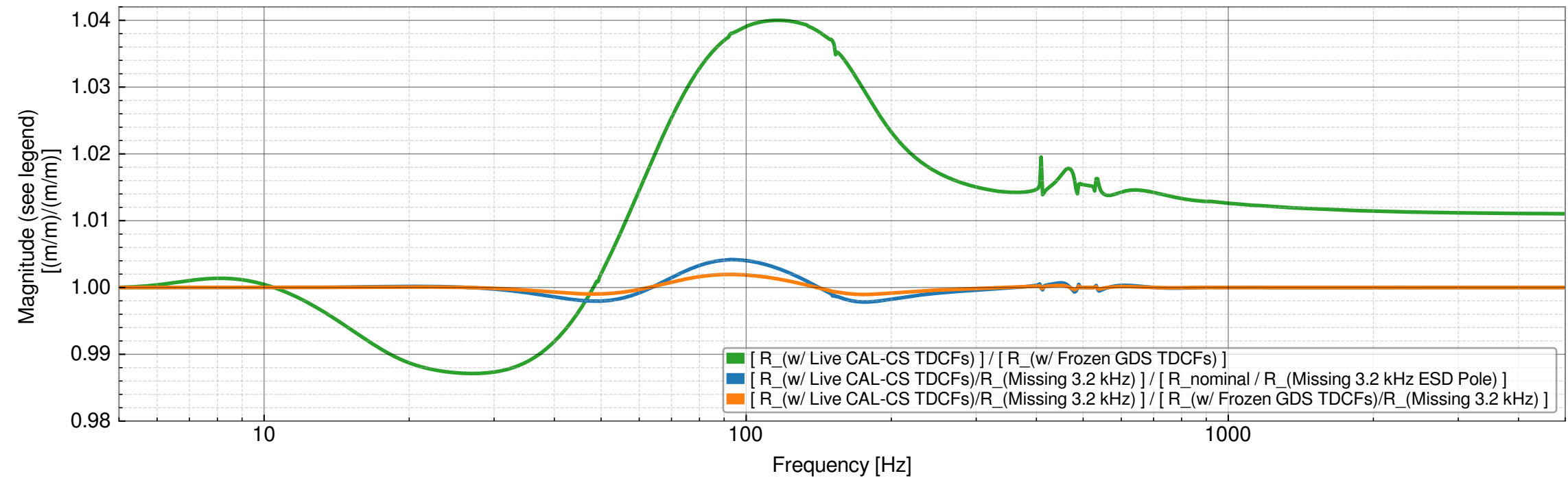
Systematic Error Comparison: Ratio of R_(w/ CALCS TDCFs) / R_(w/ GDS TDCFs) with and without Missing 3.2 kHz ESD Pole LHO:72622; NOT THERMALIZED
